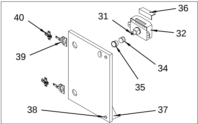
DOOR HARDWARE
