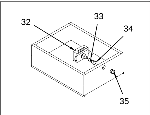
DRAWER HARDWARE
