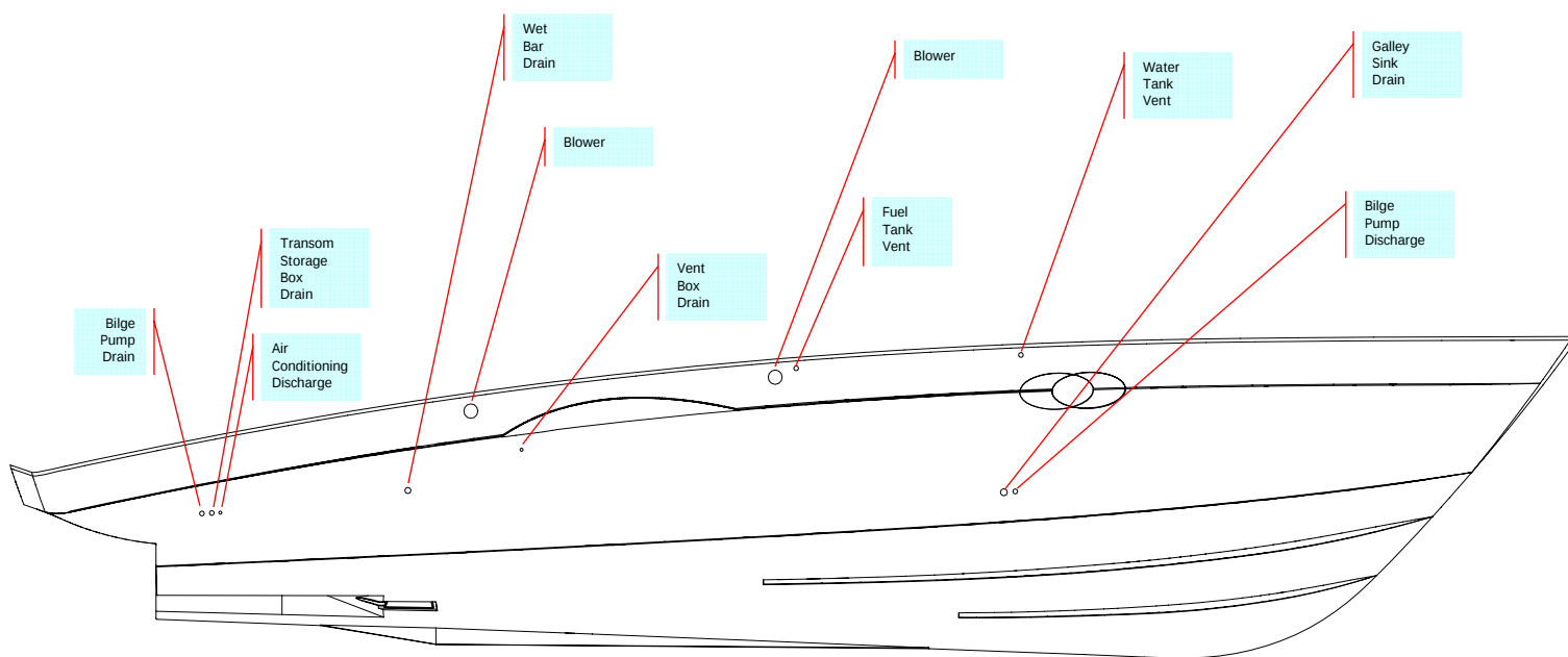
35 MOTOR YACHT THRU HULLS STARBOARD
