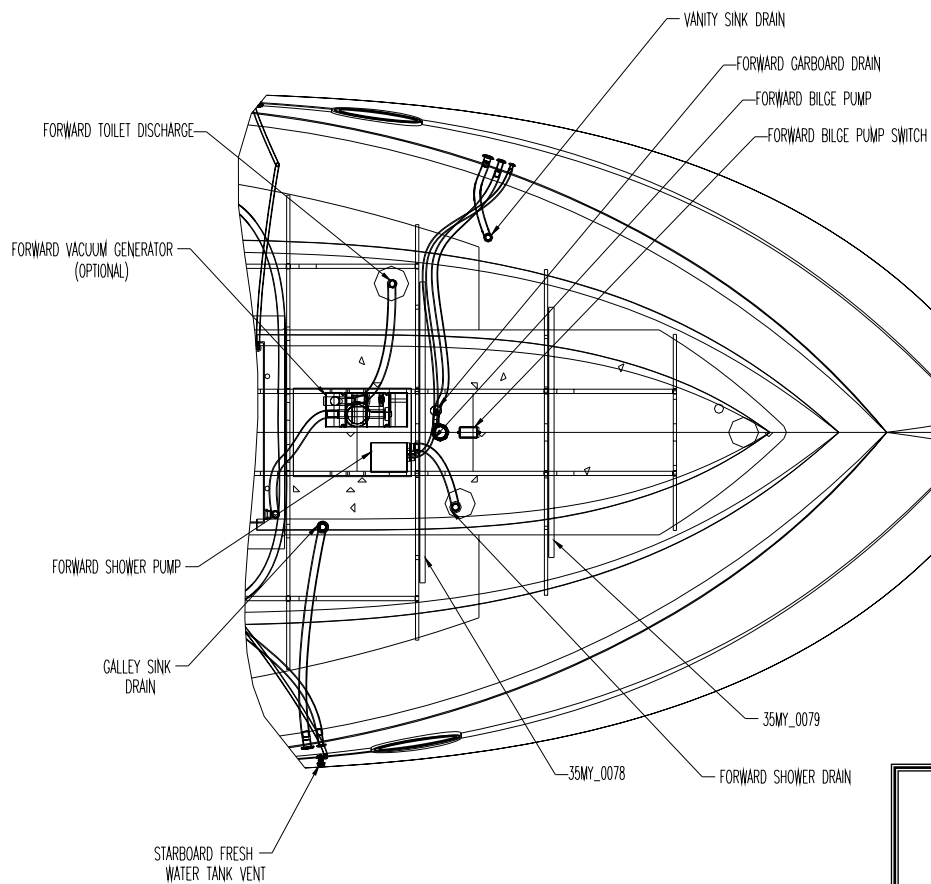
35 MOTOR YACHT Mechanical Arrangement Detail C
