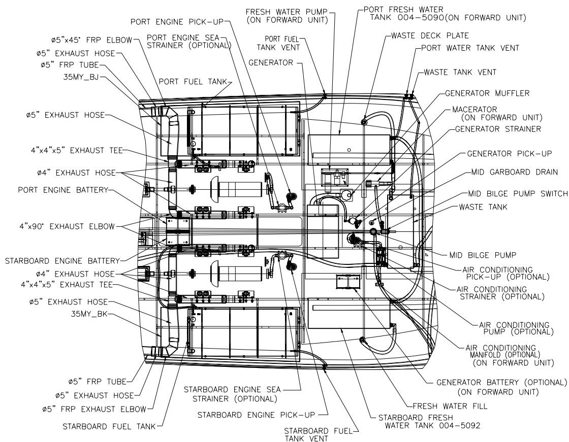
35 MOTOR YACHT Mechanical Arrangement Detail B
