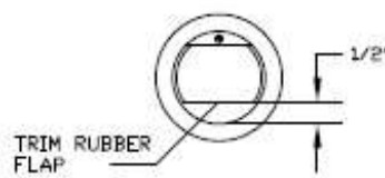
DETAIL A MODIFIED SCUPPER PN 100106
