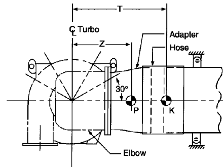
Horizontal side air inlet
