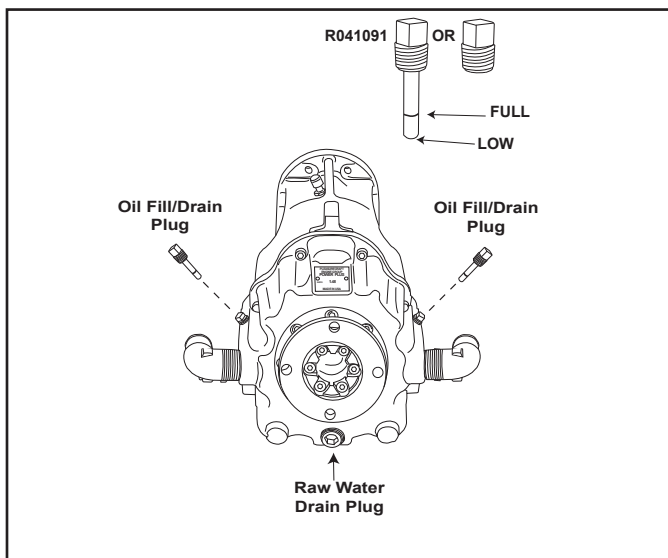
Figure 11-22 Challenger V-Drive
