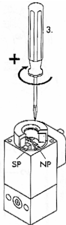
Fig 4. Adjustment of zero and span
