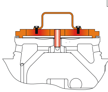
(b) Cylinder Head
