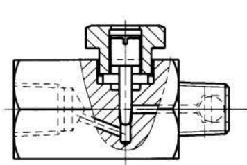
Fig.2 ) Sectional drawing
