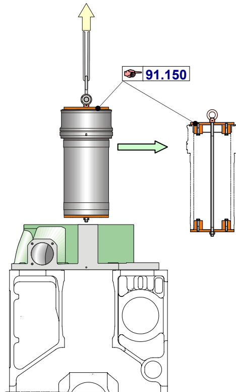
(b) Lifting of cylinder liner by lifting tool
