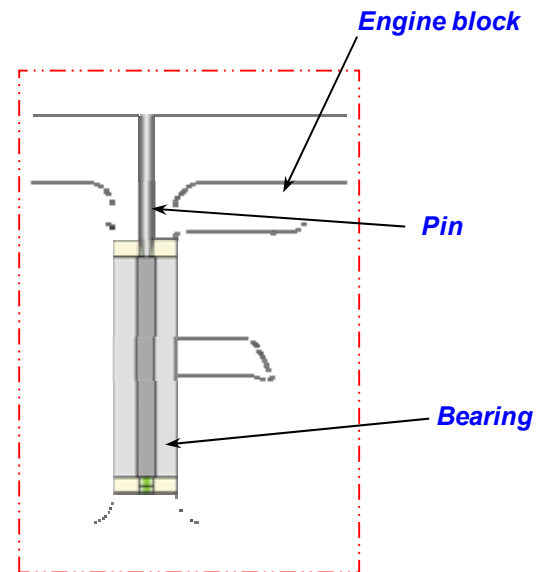
Fig.3 Pin for fixing camshaft bearing
