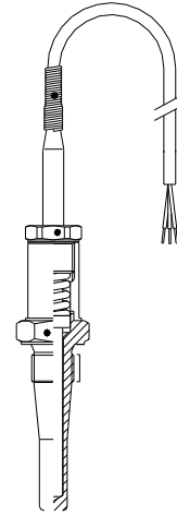
Temperature transmitter PT-100 Ω (type B)
