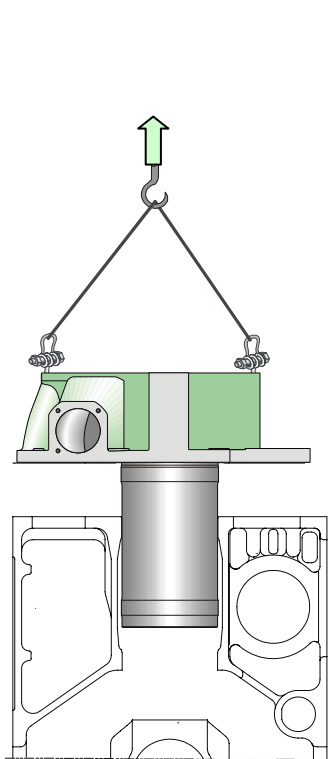
(a) Lifting of cylinder liner by water jacket
