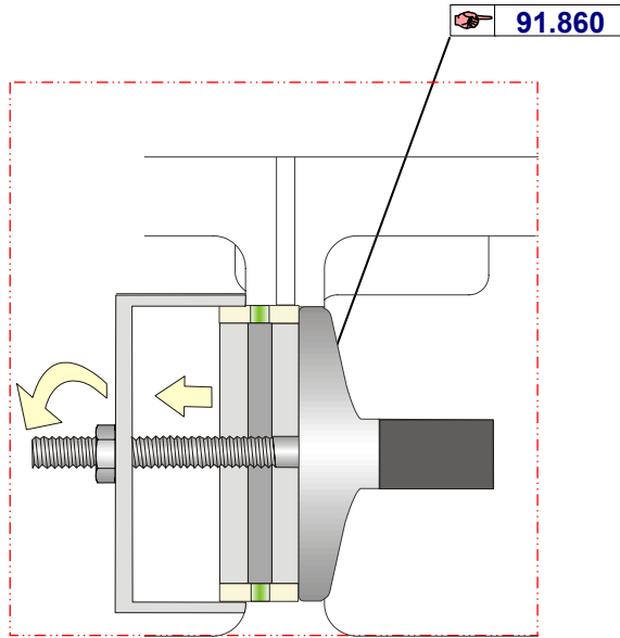
Fig.2 Extracting of camshaft bearing by tool
