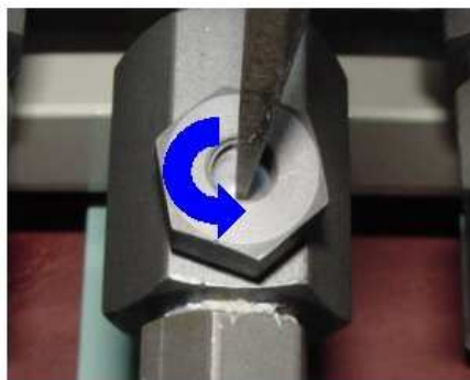
Fig.6) Adjusting the spindle
