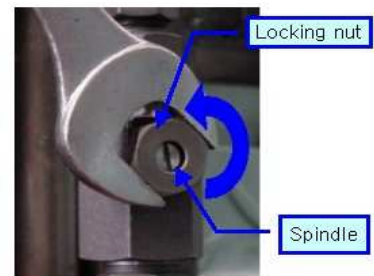
Fig.4) Loosening locking nut
