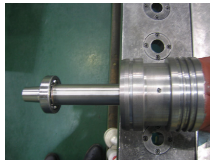
Fig.5 Assembly of sub-assembled shaft into pump housing (서버조립된 축을 펌프하우징에 조립)
