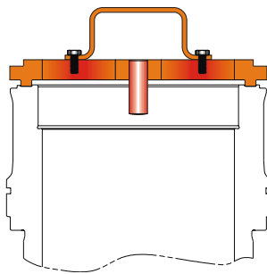
(a) Cylinder Liner
