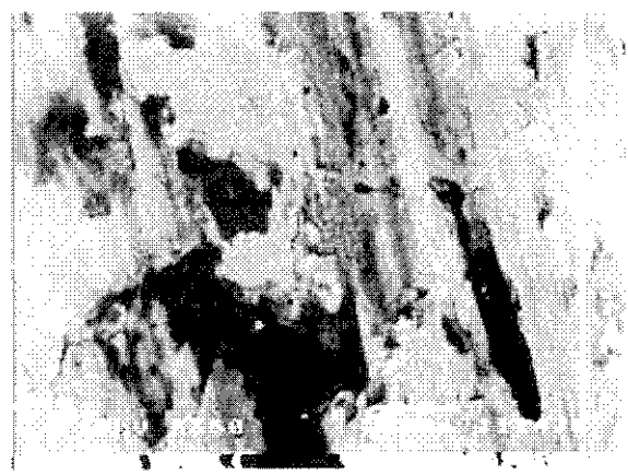
Fig. D: Magnification of scuffing marks and carbides (290x)
