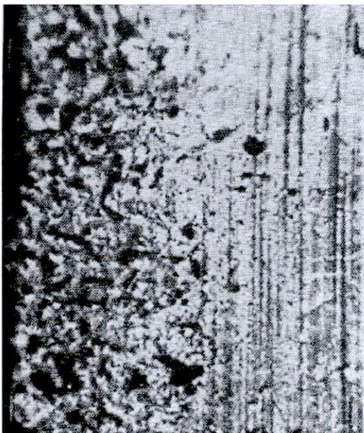
Photo 1 (X30) Typical erosion or sand-blasting on the part of the ring topside which protrudes out of the groove. This is due to hard grains being blown down through the gap in the ring above (NB: The rings "turn" in the grooves). Such erosion is only seen on rings Nos. 2, 3 and 4.
