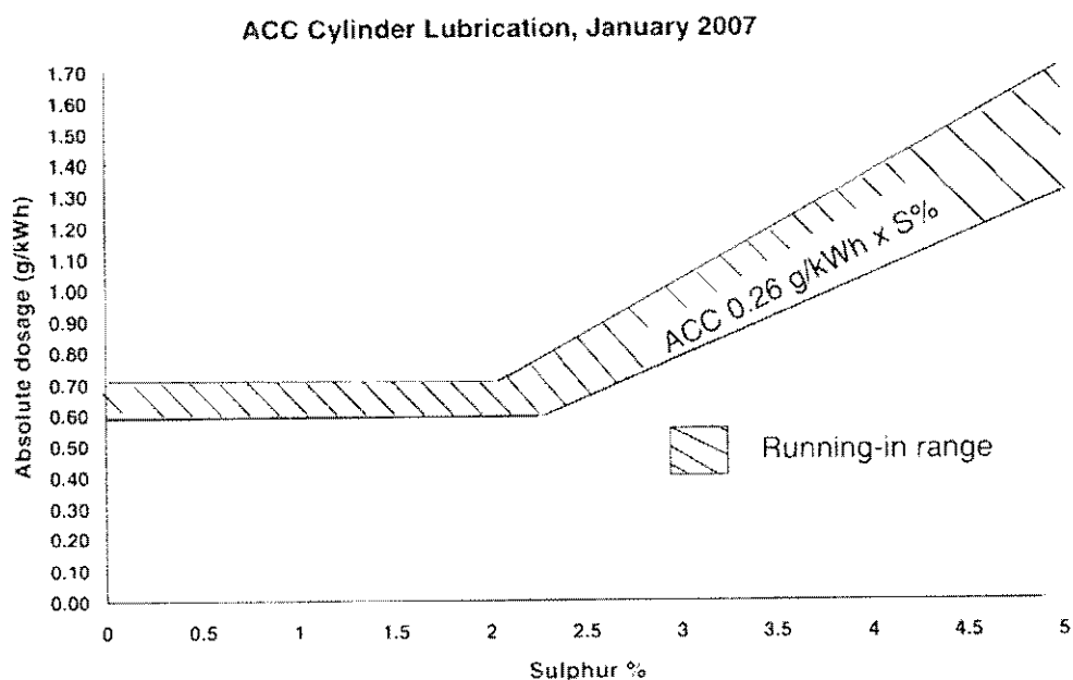
Fig. 1: ACC Cylinder Lubrication. January 2007
