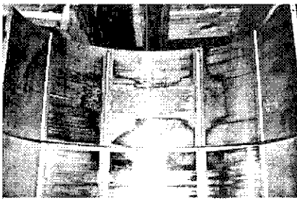
Initial scuffing of Ni-layer
