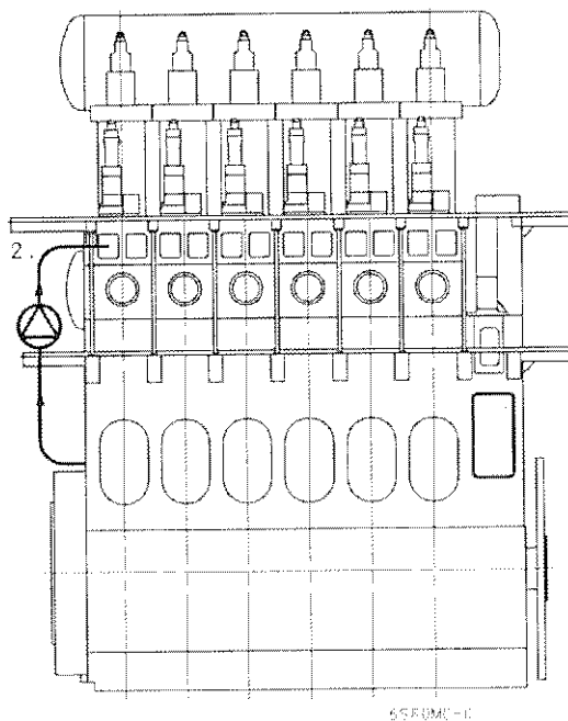
System 2 View from exhaust side
