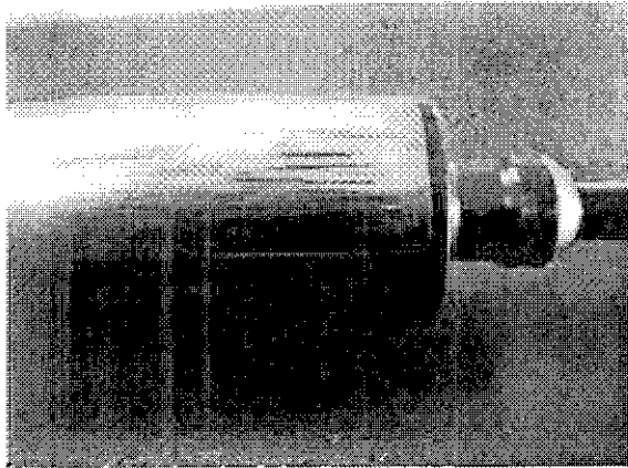
Fig. A: Fuel valve cut-off shaft with scuffing marks
