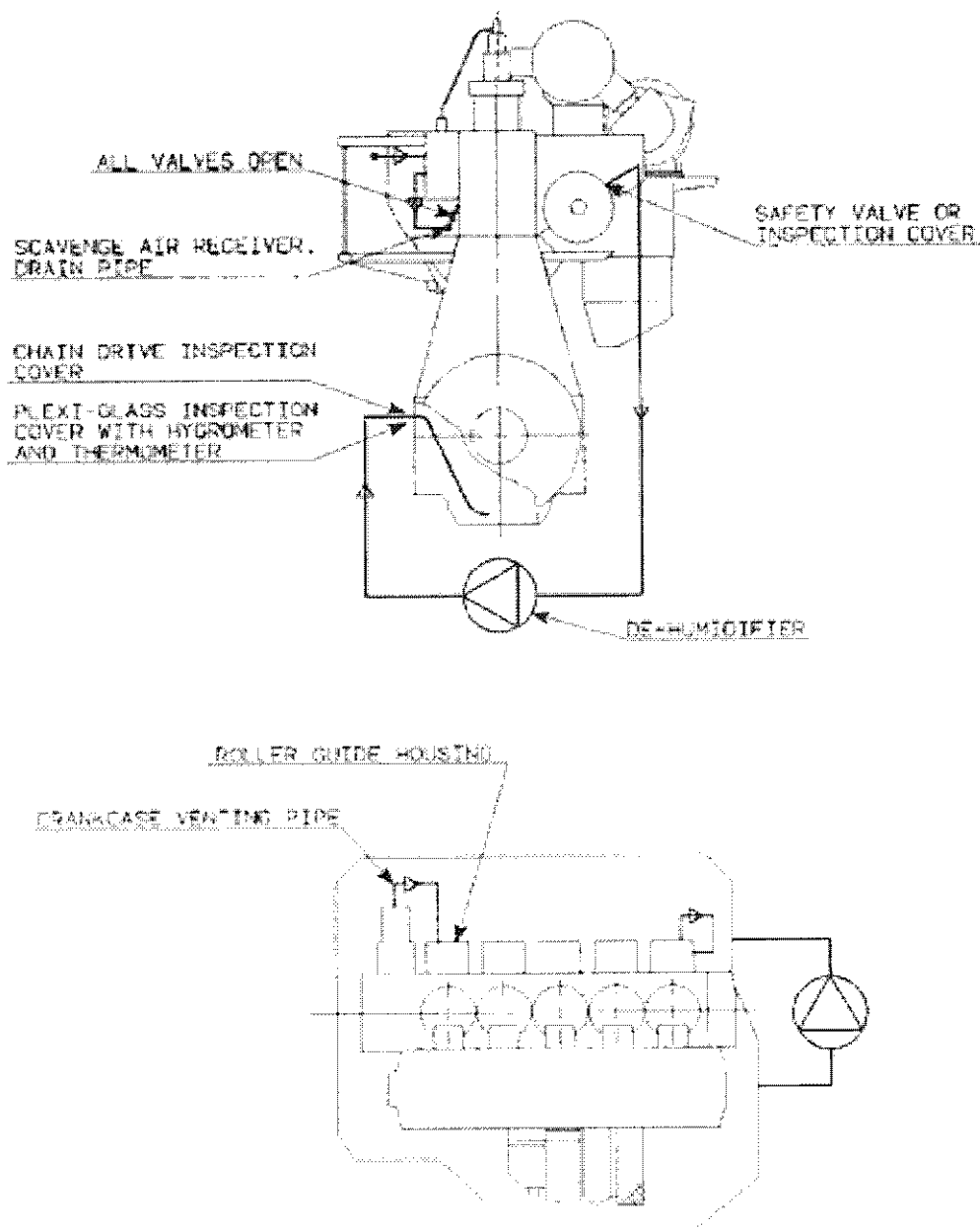
Figure 1 Diagram of connection of dehumidifier.
