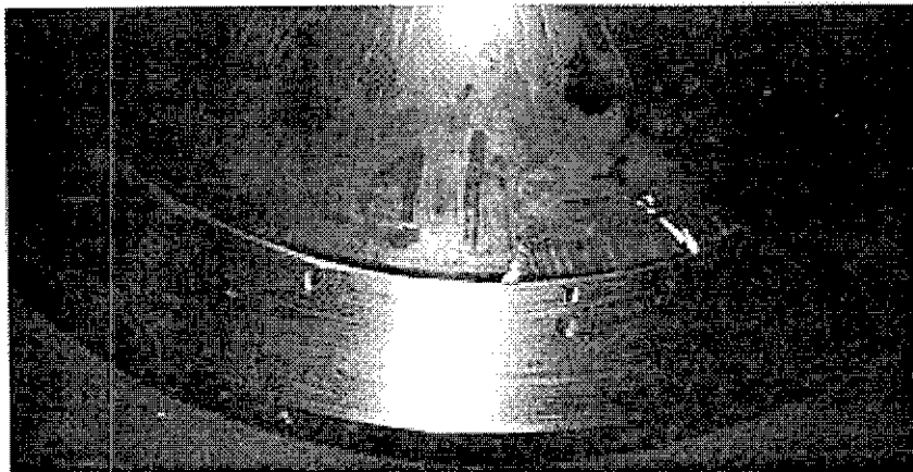
Photo 5: Acceptable seat condition after grinding
