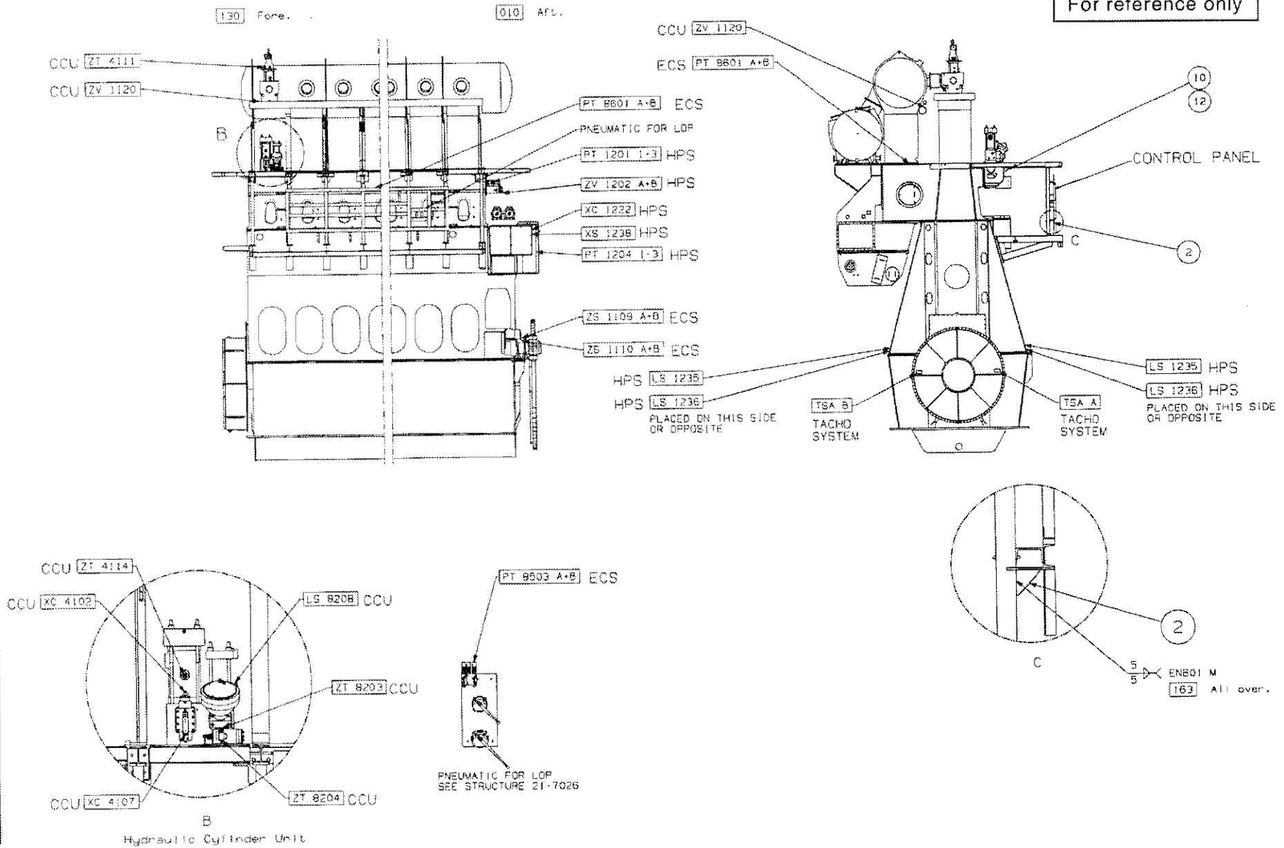
Figure 2: Location of Basic Measuring Points
