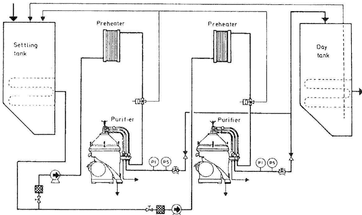
In Parallel
