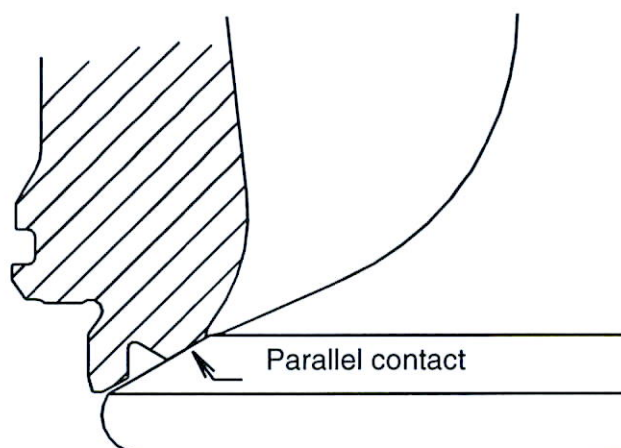
Fig. 2: Contact condition during running
