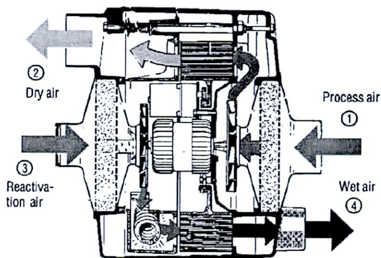
Figure 6 Examples of dehumidifiers
