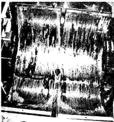
Bearing metal worn out, steel-steel contact
