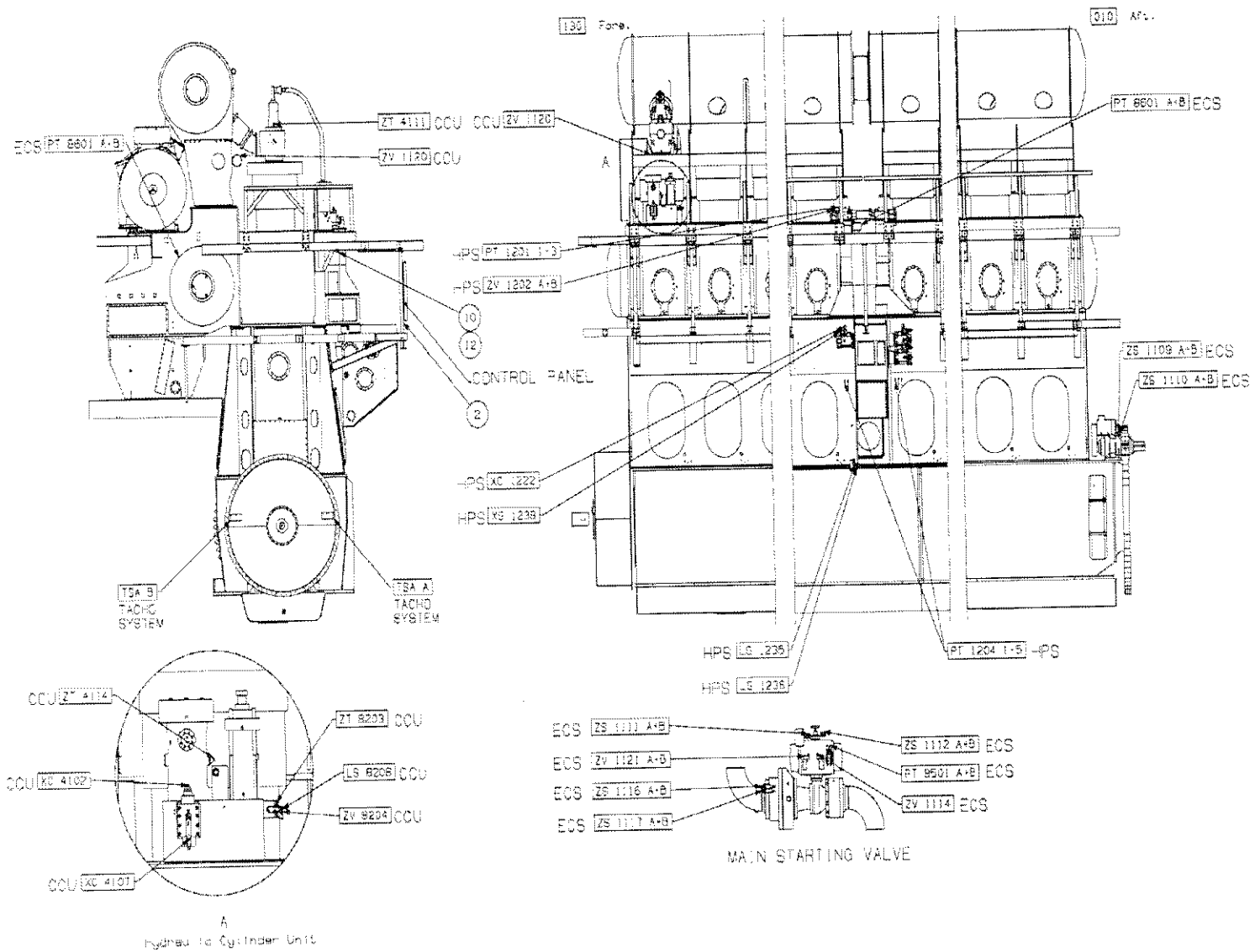
Figure 3: Location of Basic Measuring Points
