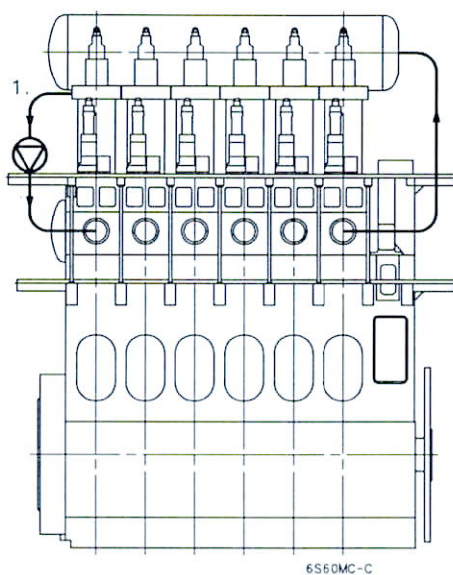
System 1 View from exhaust side
