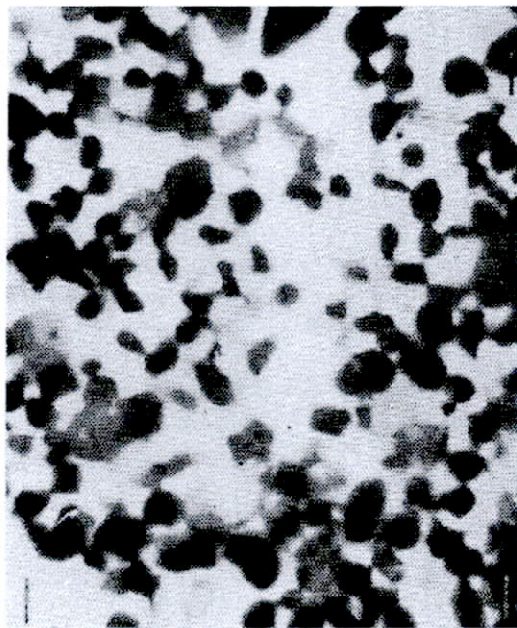
Photo 3 (X250) Sand (or sand-like grains) separated from centrifuge sludge . In this case the centrifuge treated the fuel oil after the oil had passed a full flow (fabric) filter. The particles size is 10 \mu to 15 \mu .
