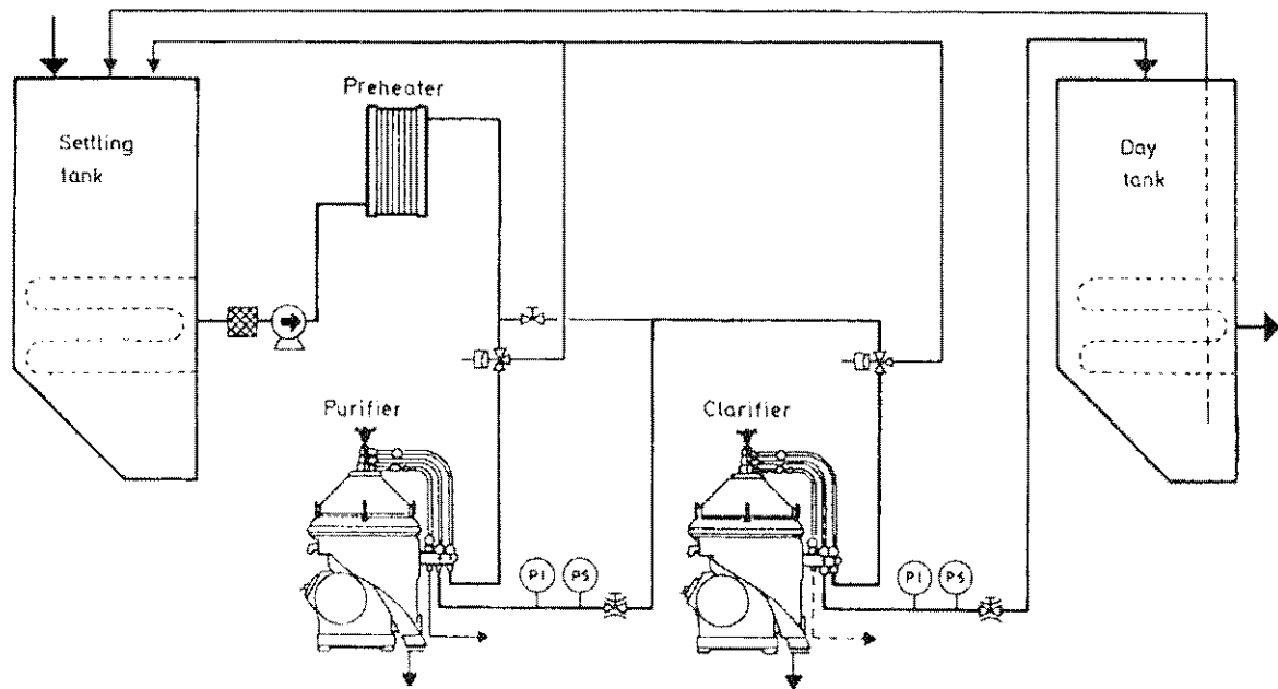
In Series
