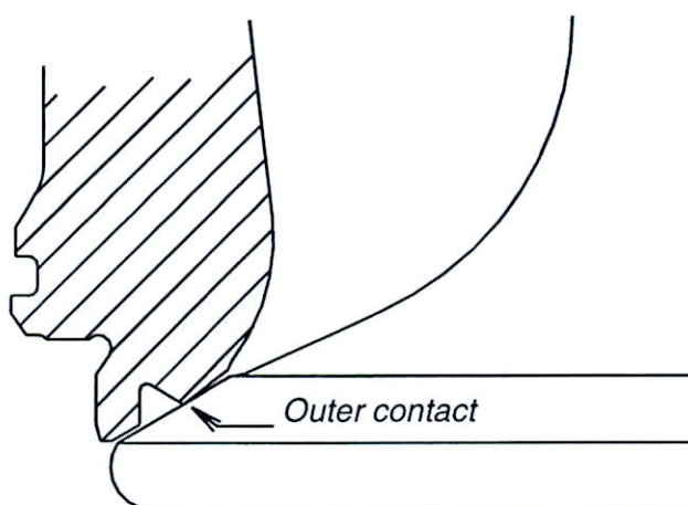
Fig. 3: Outer contact, increased risk of blow-by
