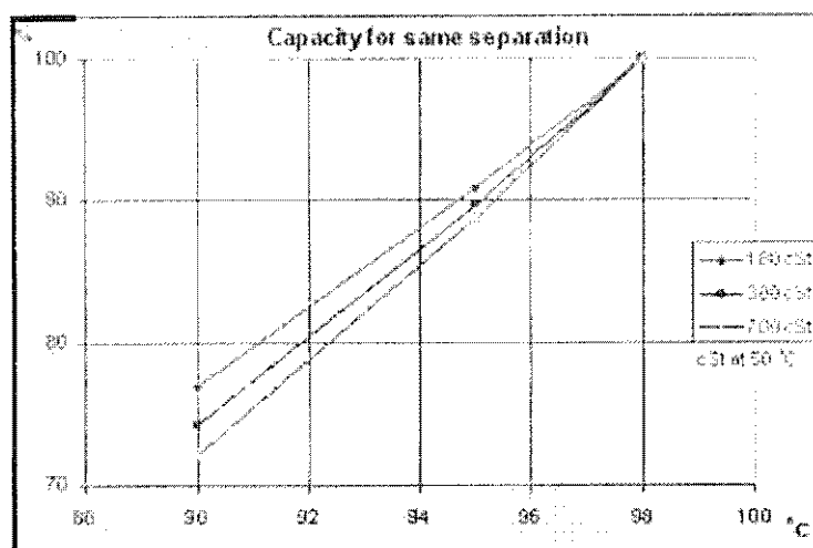
Fig. 1: Relationship between throughput and temperature
