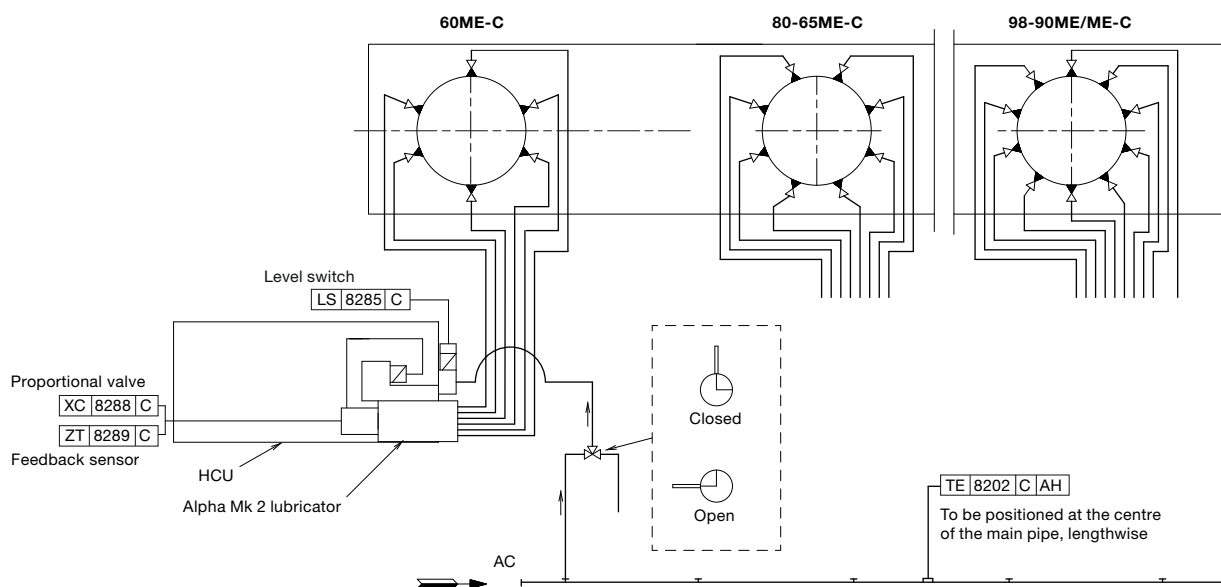
Fig. 9.02.04a: Cylinder lubricating oil pipes, Alpha/ME lubricator
