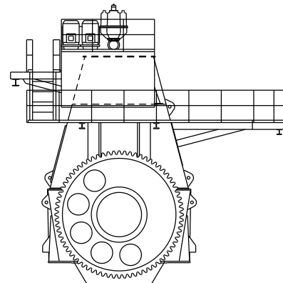
Fig. 19.03.01: Dispatch pattern, engine with turbocharger on exhaust side (4 59 123)
