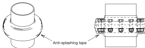
Fig. 7.04.04b: Anti-splashing tape (FN tape)
