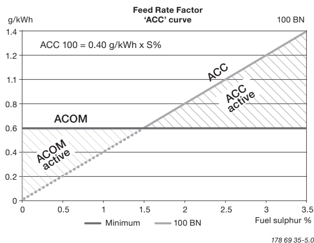
Fig. 9.01.01: Mixing principle, ACOM
