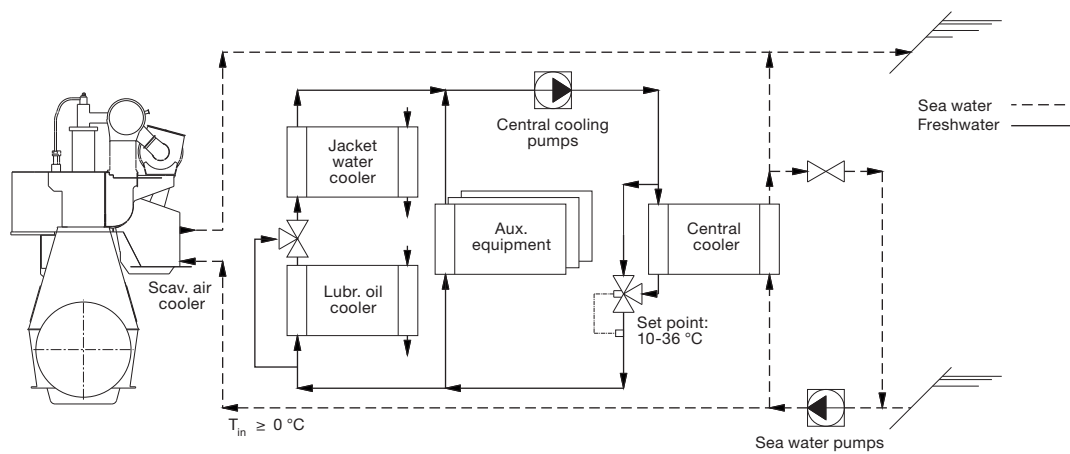
Fig. 11.01.01c: Principle diagram of combined cooling water system
