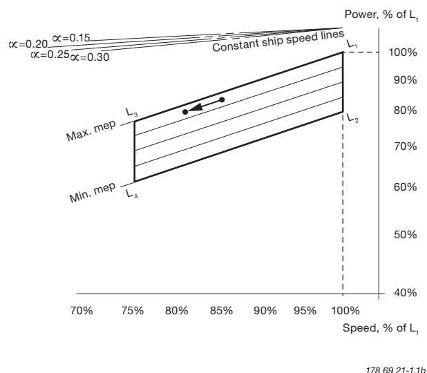
Fig. 2.05.03b: Layout diagram. Power and speed derating but no MEP derating, SFOC is unchanged
