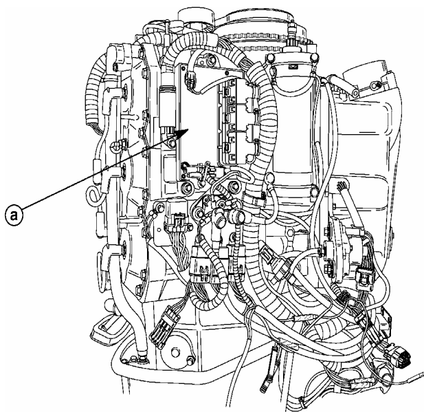
a) Electronic Control Module (ECM)
