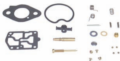
18-7226 CARB KIT Replaces: 1395-9650 Fits: 30 JET, 40/45 4 CYL 4 Stroke, Carb models WMA-7B,9,10,13
