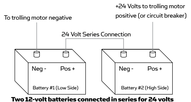
Two 12-volt batteries connected in series for 24 volts
