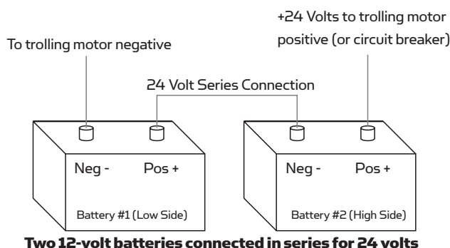
Two 12-volt batteries connected in series for 24 volts
