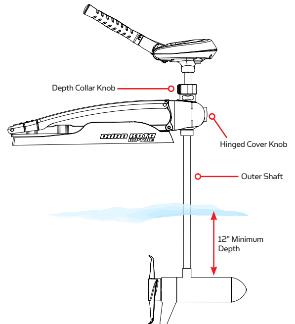
Latch & Door Models
