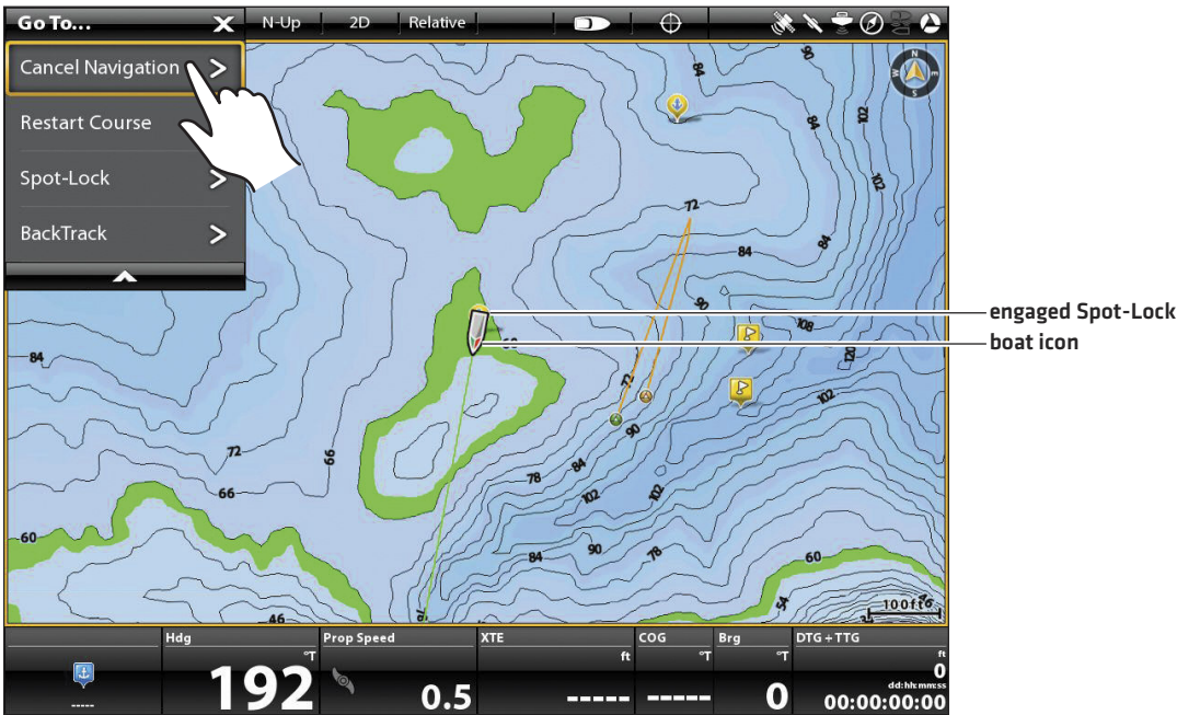
Canceling Spot-Lock Navigation (ONIX)
