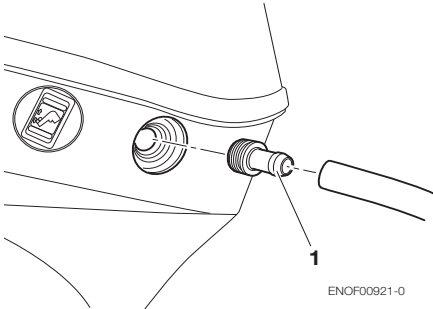
1. Flushing attachment
