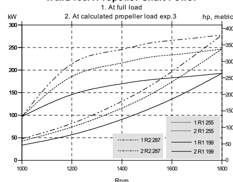
TAMD103A Torque
