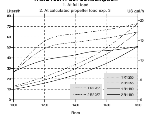
TAMD103A Fuel Consumption
