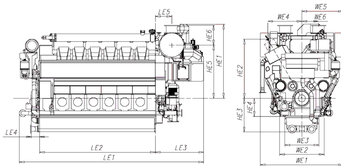
Fig 1-4 V-engines (DAAF066203)
