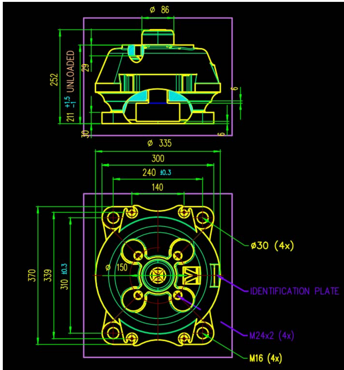
Fig 15-12 Rubber mount, V-engines (DAAE018766C)
