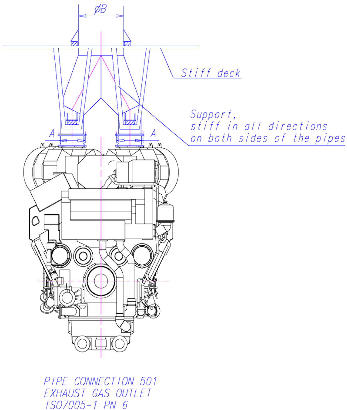
Fig 11-5 Exhaust pipe, diameters and support (DAAF068200B, DAAF068204B)
