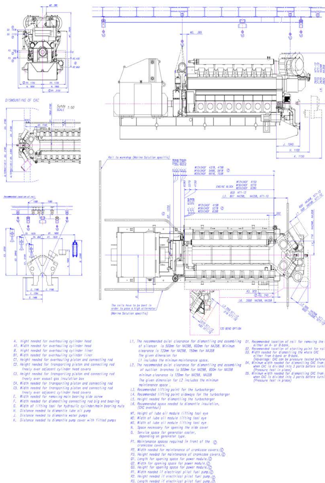
Fig 18-14 Service space requirement, genset (DAAF066517C)
