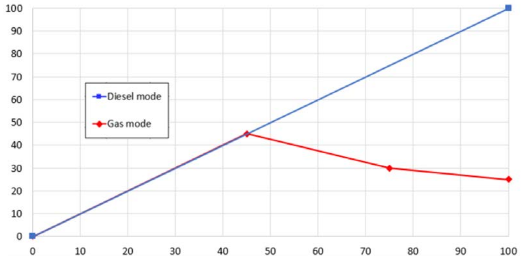
Fig 2-6 Maximum instant unload decrease [%]
