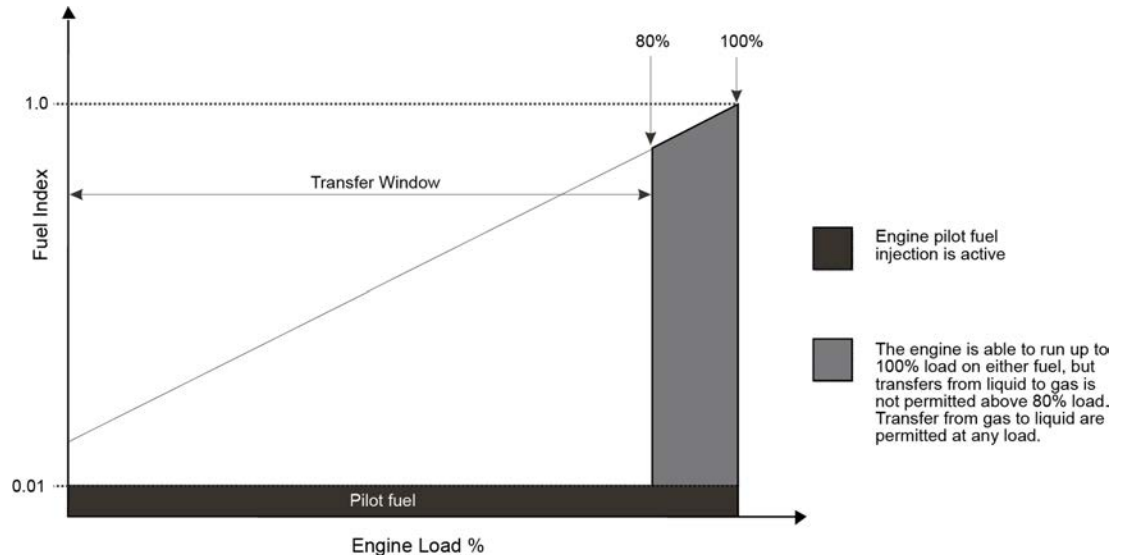
Fig 14-8 Operating modes are load dependent
