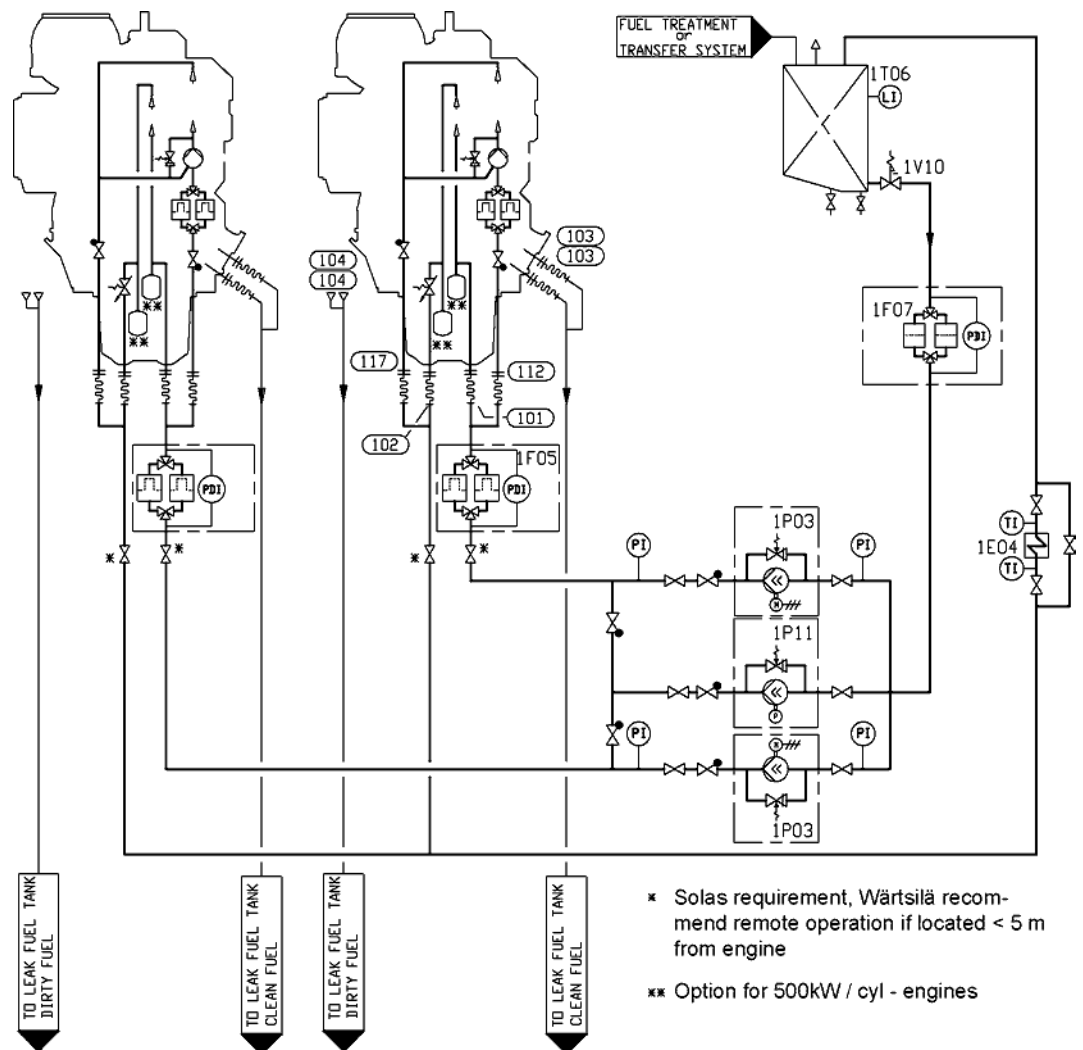
Fig 6-14 Example of fuel oil system (MDF) multiple engine installation (DAAE085364C)
