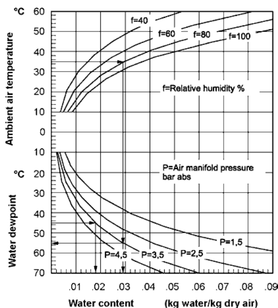
Fig 10-3 Condensation in charge air coolers
