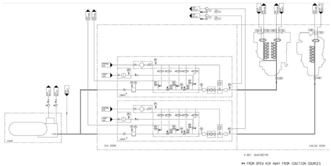
Fig 6-3 Example of fuel gas operation with open type GVU (DAAF022750G)
