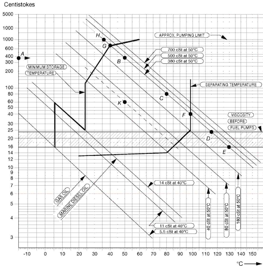
Fig 6-11 Fuel oil viscosity-temperature diagram for determining the pre-heating temperatures of fuel oils (4V92G0071b)
