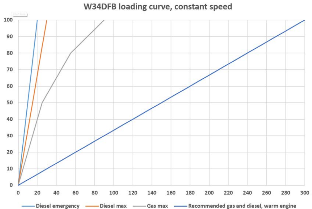
Fig 2-3 Constant speed applications
