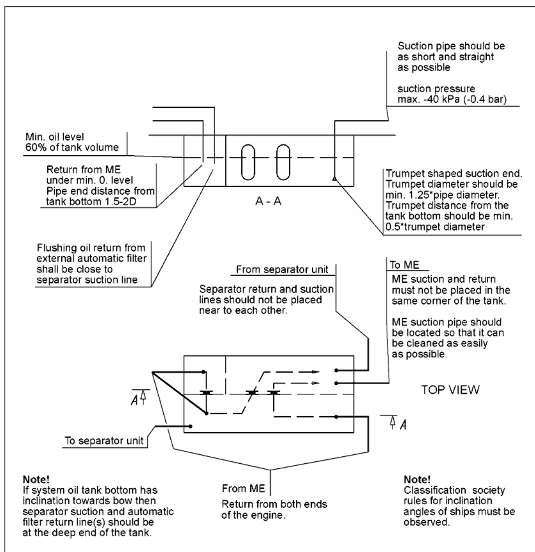
Fig 7-7 Example of system oil tank arrangement (DAAE007020e)
