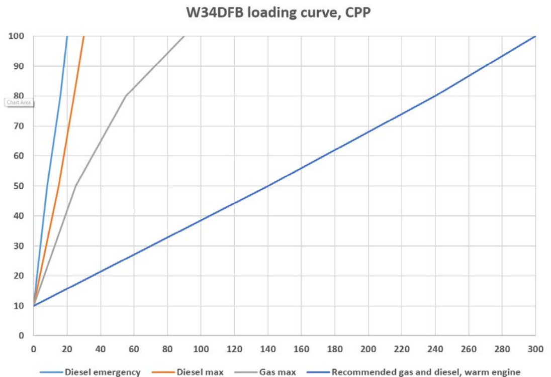
Fig 2-2 Variable speed, controllable pitch propeller (CPP)
