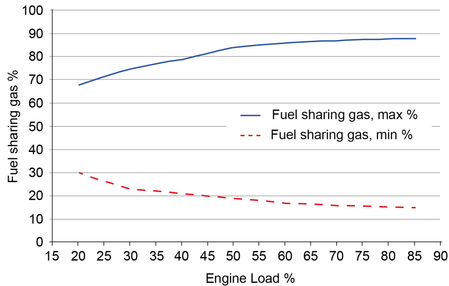
Fig 14-7 Fuel mixing ratio
