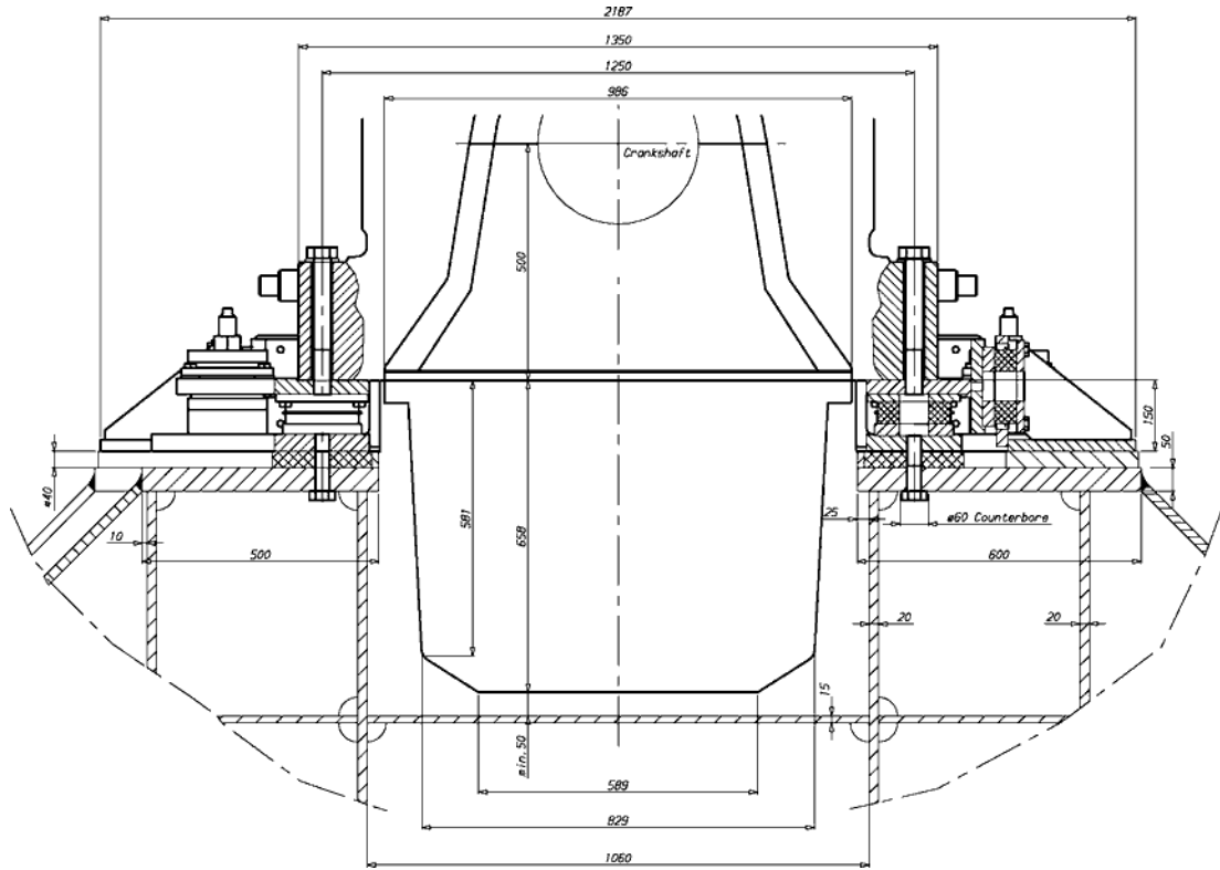
Fig 15-6 Principle of resilient mounting, W9L34DF (V69A0247A)
