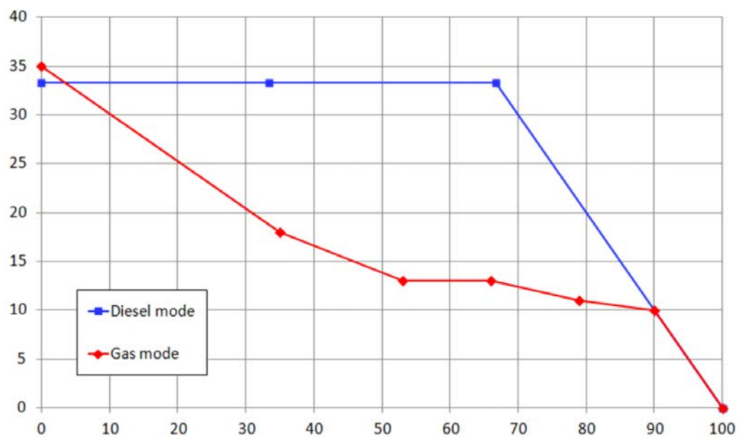
Fig 2-5 Maximum instant load increase [%]
