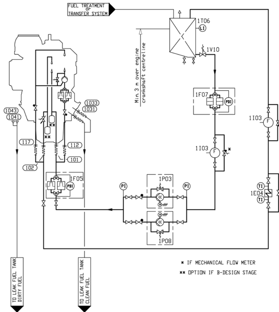
Fig 6-13 Example of fuel oil system (MDF), single engine installation (DAAE055756D)
