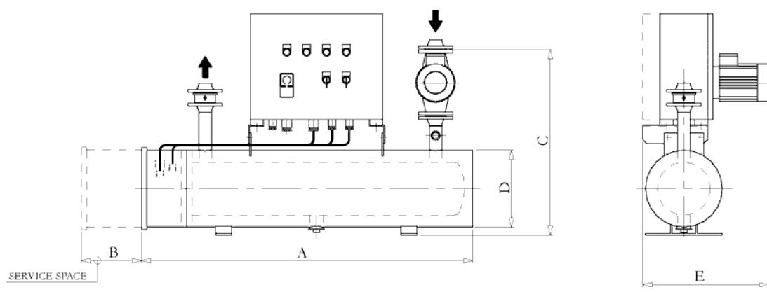
Fig 9-8 Preheating unit, electric (3V60L0562C).
