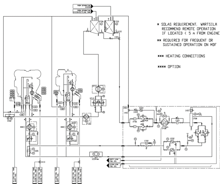
Fig 6-15 Example of FO system (HFO), multiple engine installation (DAAE085365G)
