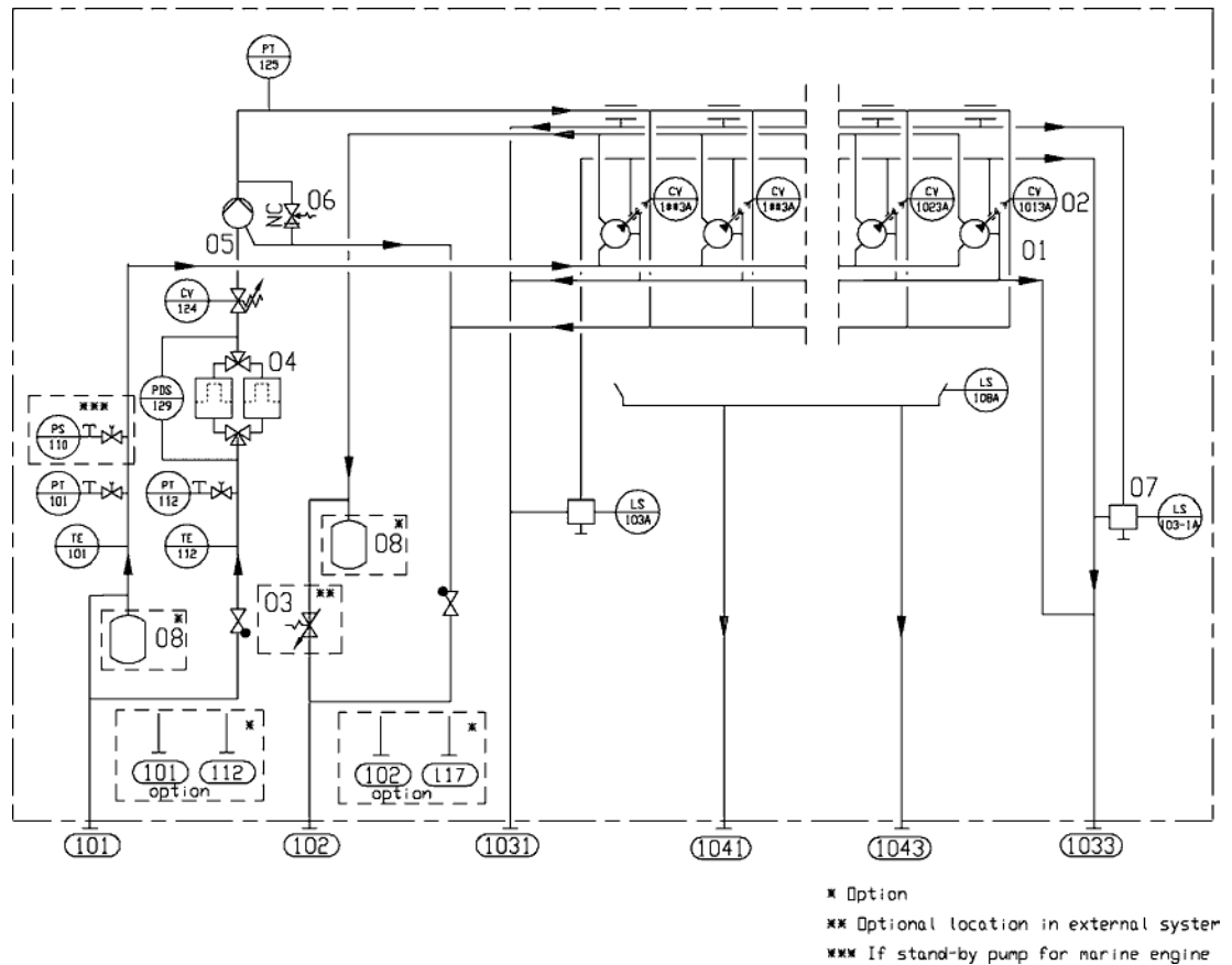
Fig 6-8 Internal fuel oil system for inline engines, LFO (DAAF282780A)
