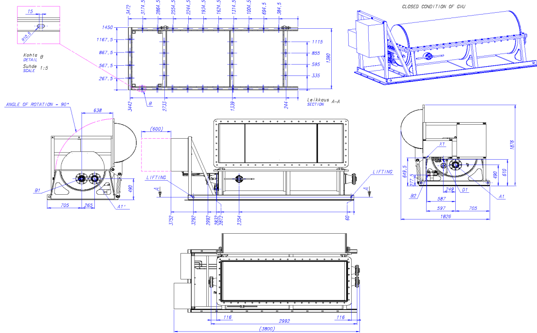
Fig 6-7 Main dimensions of the GVU (DAAF020519A)
