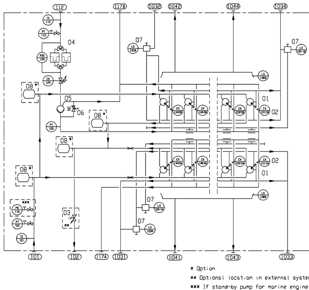
Fig 6-10 Internal fuel oil system for V-engines (DAAF283159)
