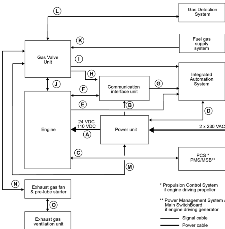
Fig 14-3 UNIC C3 overview
