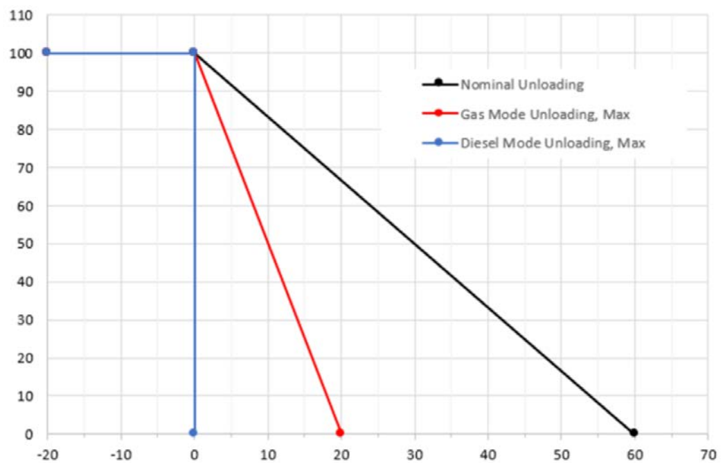
Fig 2-4 Unloading, Constant speed and CPP applications
