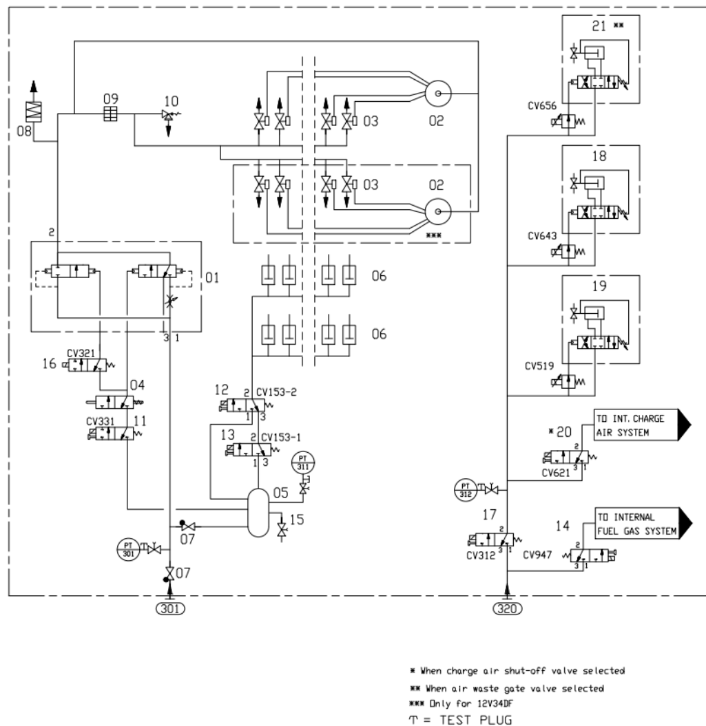
Fig 8-2 Internal compressed air system for V-engines (DAAF283527A)
