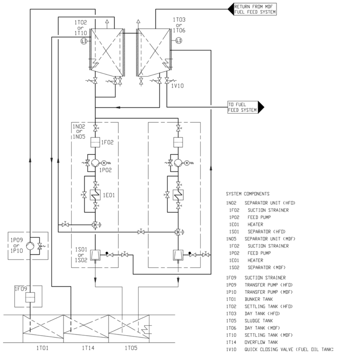
Fig 6-12 Fuel transfer and separating system (V76F6626G)
