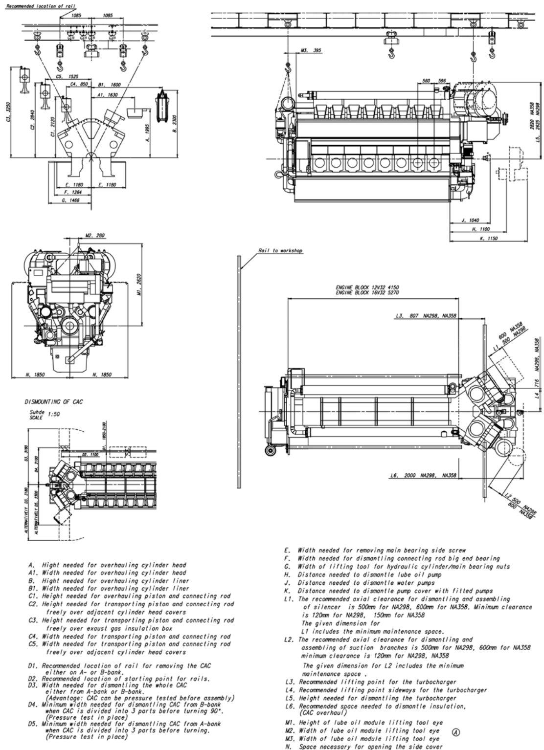
Fig 18-13 Service space requirement, turbocharger in free end (DAAF066536)
