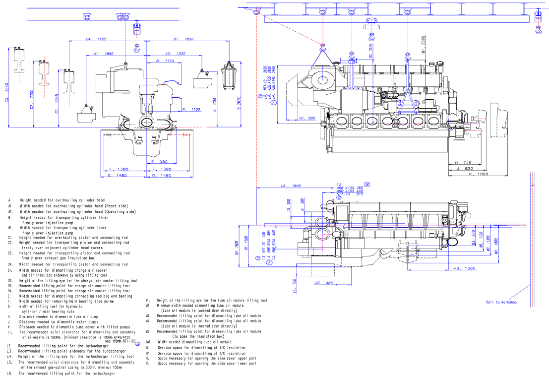
Fig 18-10 Service space requirement, turbocharger in driving end (DAAF088437C)
