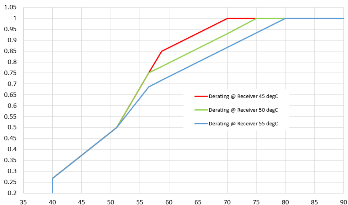
Fig 1-1 Output limitations due to methane number and charge air receiver temperature
