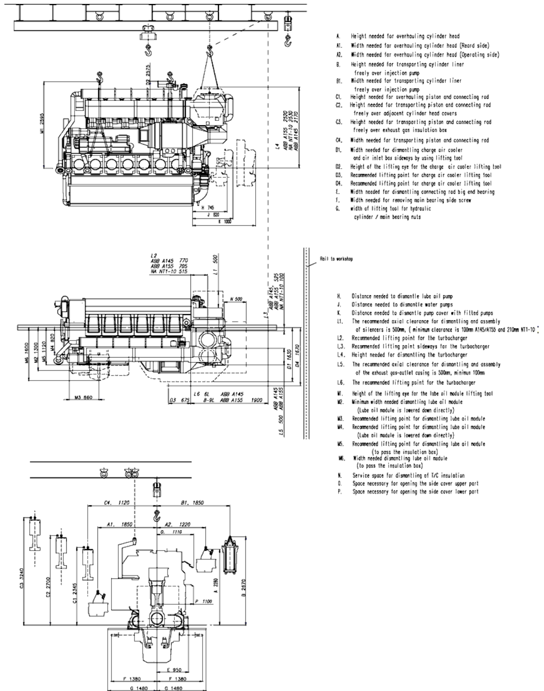
Fig 18-11 Service space requirement, turbocharger in free end (DAAF070676C)
