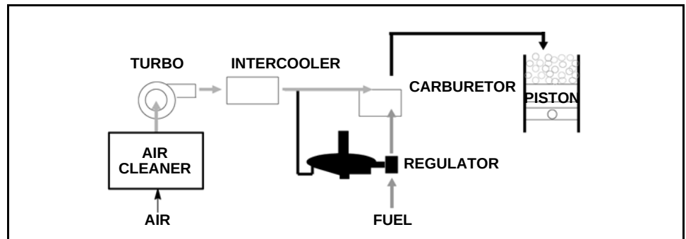
Figure 8-2 Turbocharged Engine
