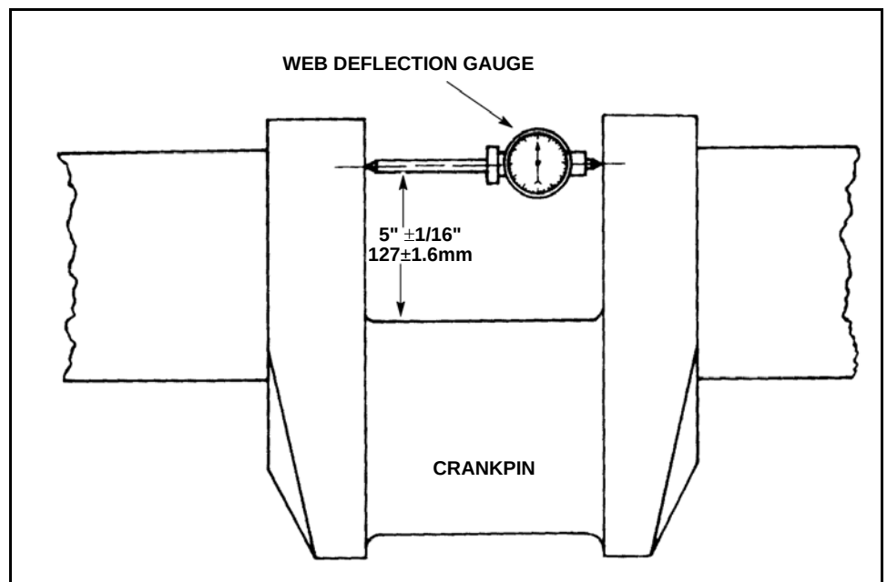
Figure 2-14 Crankshaft Web Deflection
