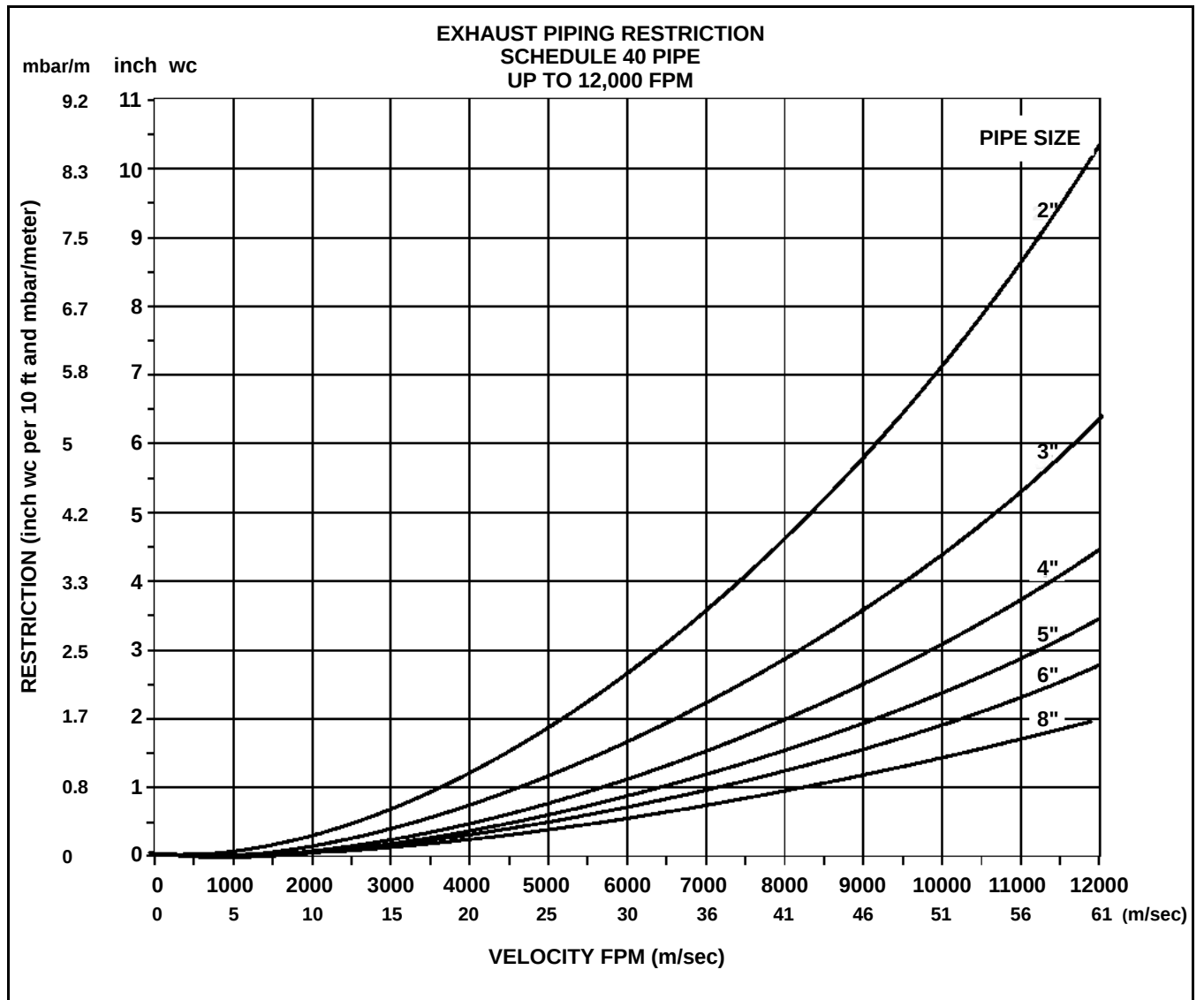
Figure 7-2 Restriction Vs. Velocity for Pipe Diameter up to 8"
