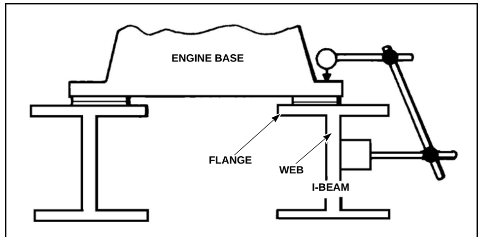
Figure 2-5 Correct Mounting
