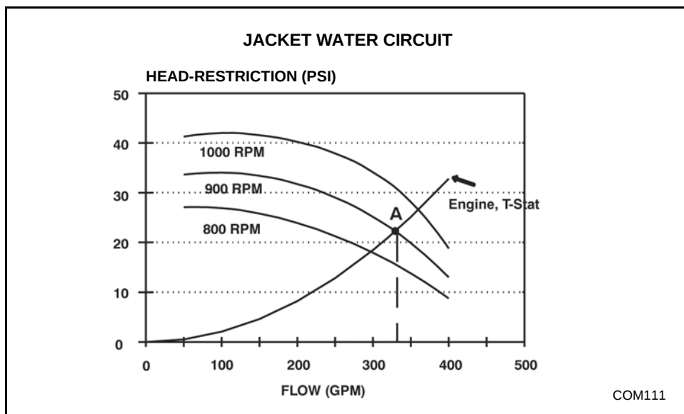
Figure 4-6 Restriction and Water Pump Outlet
