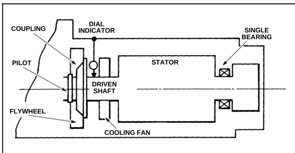
Figure 2-24 Single Bearing Generator
