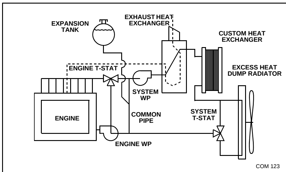
Figure 4-20 Two Pump Heat Recovery System (vent lines not pictured)
