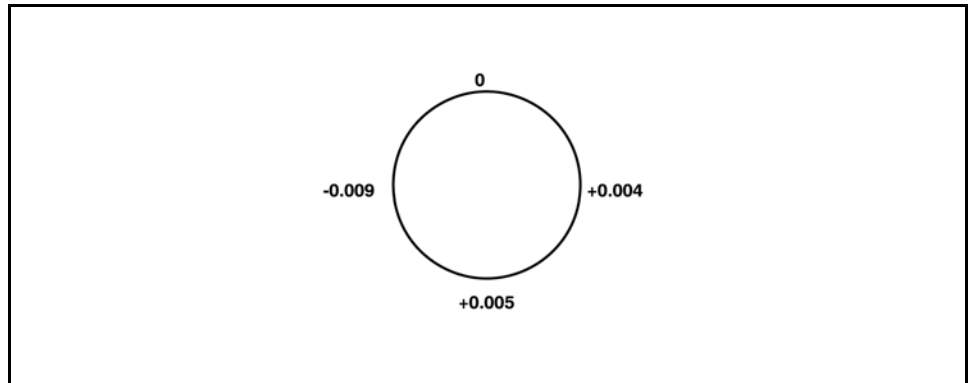
Figure 2-36 Total Indicator Reading (TIR)
