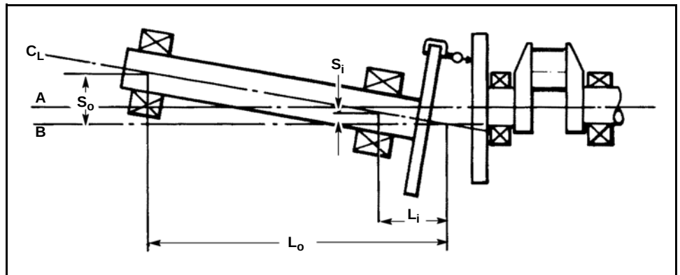
Figure 2-37 Multi-Bearing Driven Equipment
