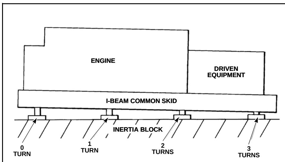
Figure 2-17 Leveling Spring Isolators
