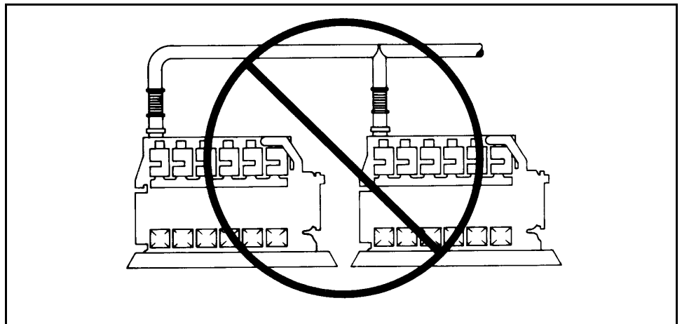
Figure 7-7 Common Exhaust System
