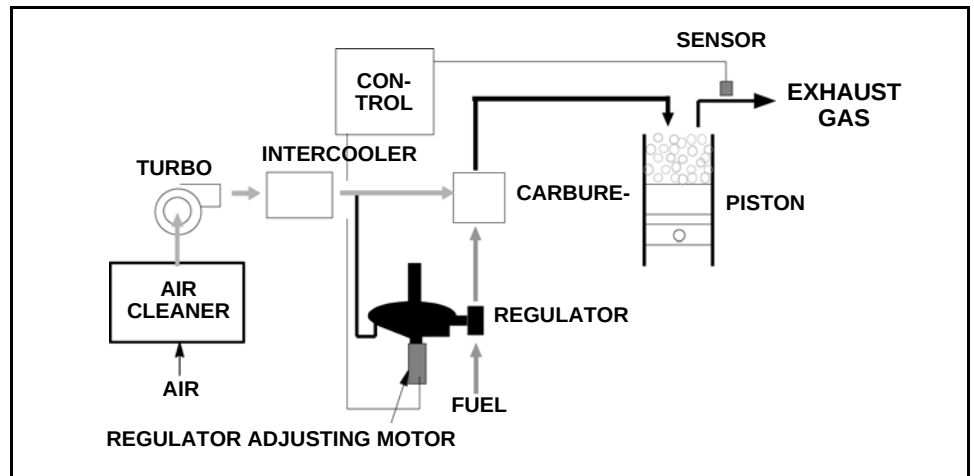
Figure 8-5 Electronic Air/Fuel Ratio Control
