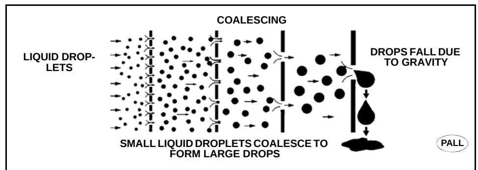
Figure 8-13 Coalescing Filter
