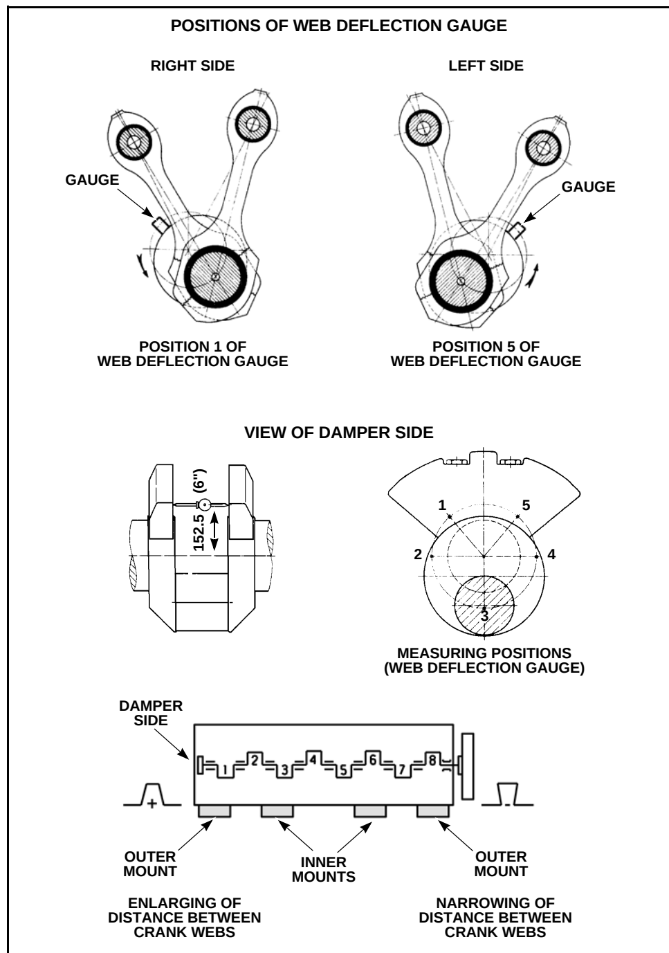
Figure 9-5 Checking The Crankshaft Deflection
