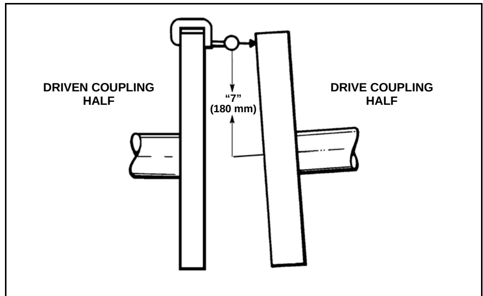
Figure 9-7 Distance from Center of Shaft to Dial Indicator
