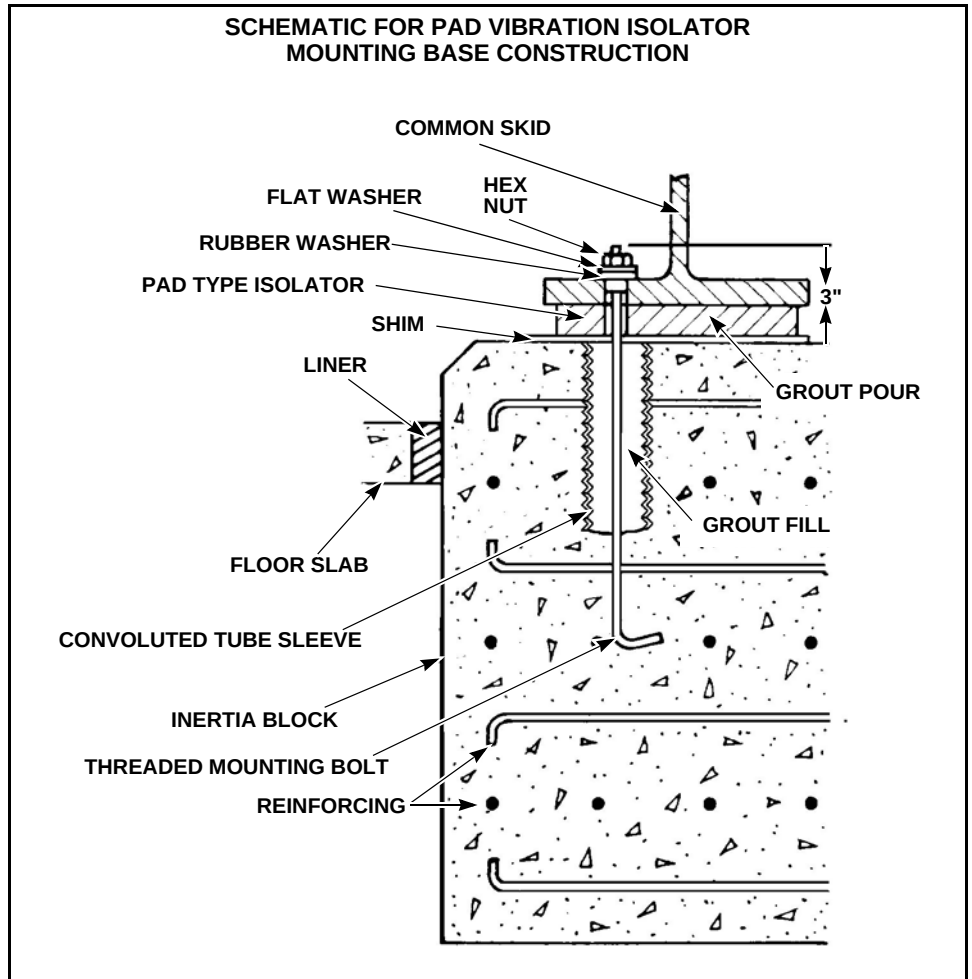
Figure 1-7 Common Skid Mounted on Pad Type Vibration Isolators
