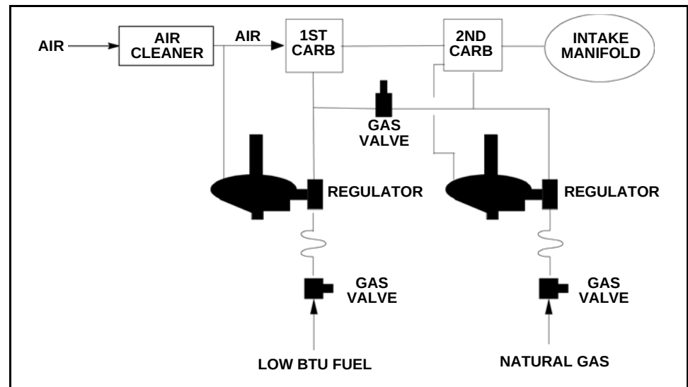
Figure 8-9 Series Carburetors
