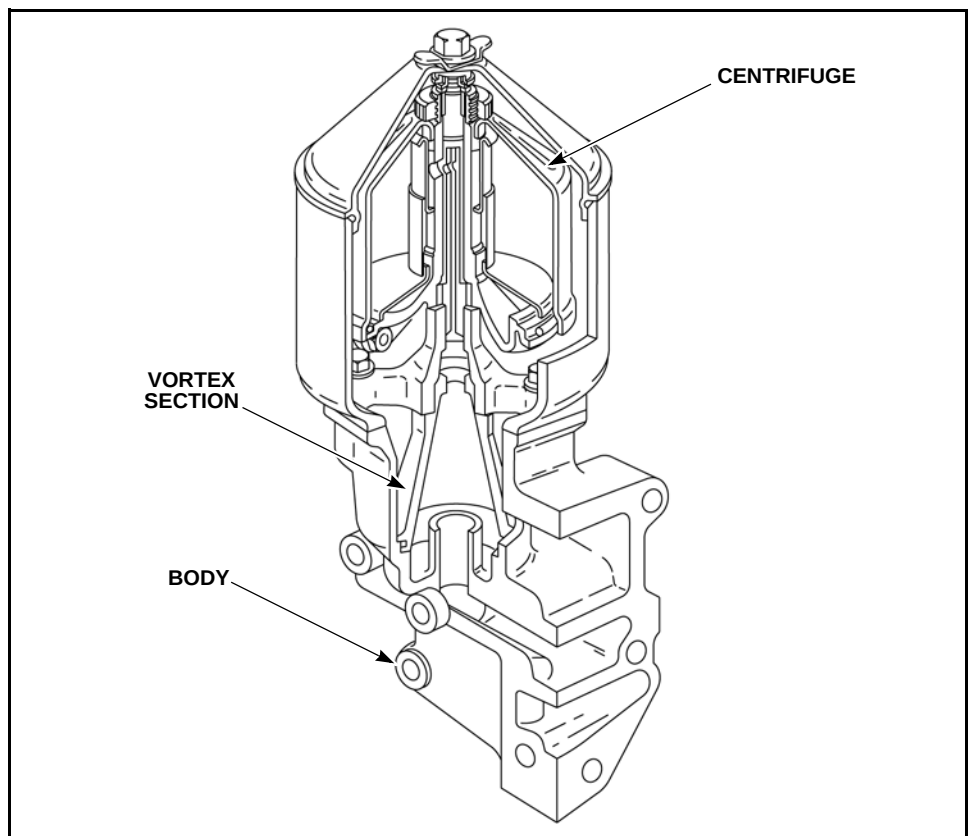
Figure 5-4 Centrifugal Oil Filter Major Sections
