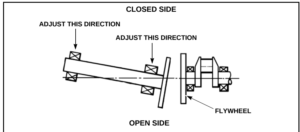
Figure 9-11 Adjusting Coupling
