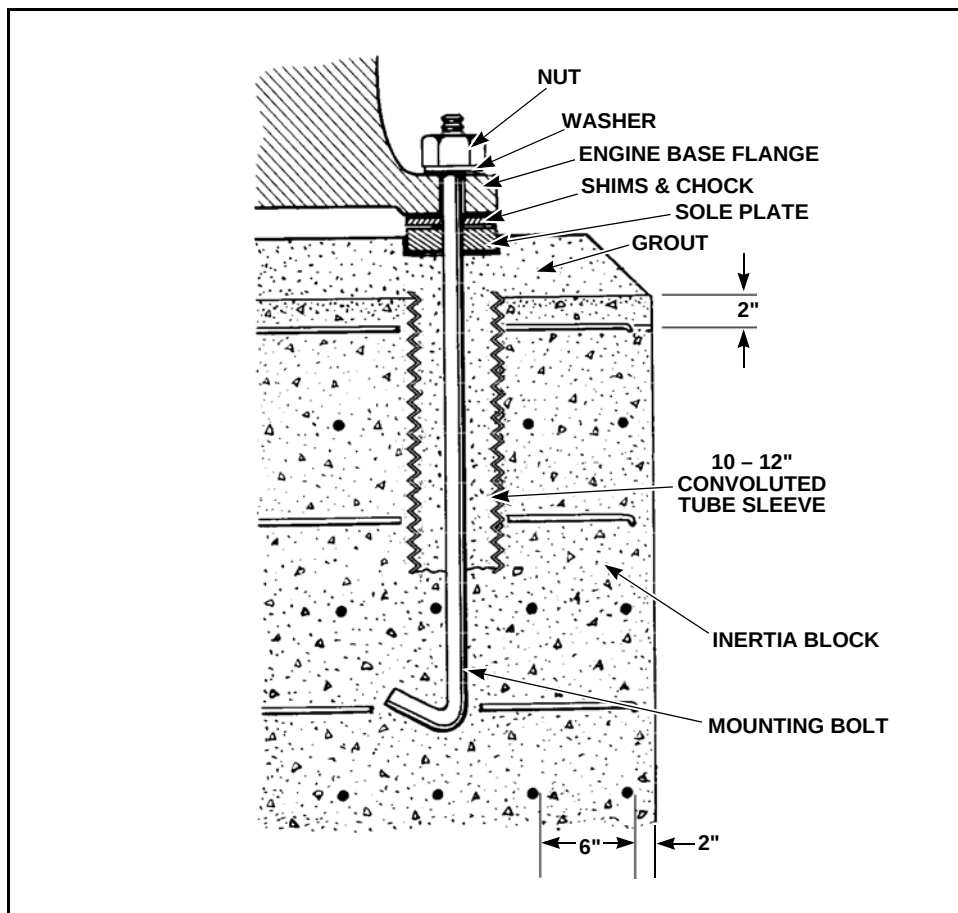
Figure 1-11 Cross Section of Mounting Using Sole Plates
