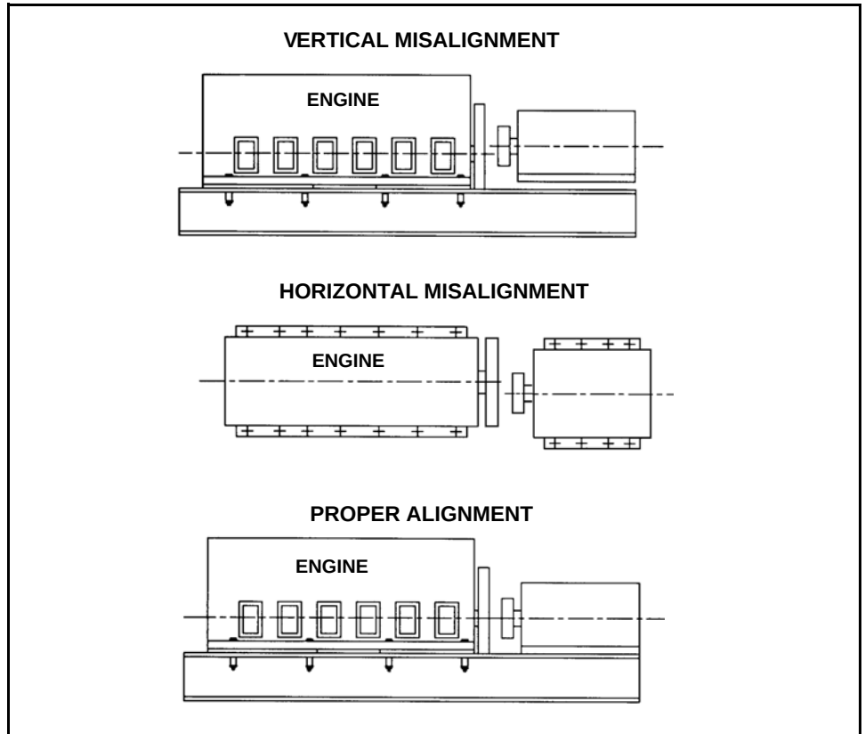
Figure 9-16 Parallel Alignment
