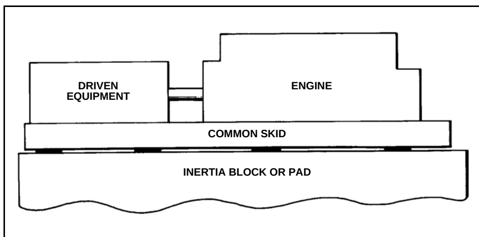
Figure 2-7 Leveling – Common Skid-to-Inertia Block
