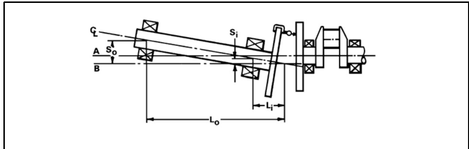
Figure 9-10 Multi-bearing Driven Equipment
