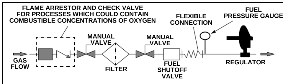
Figure 8-10 Typical Fuel Train
