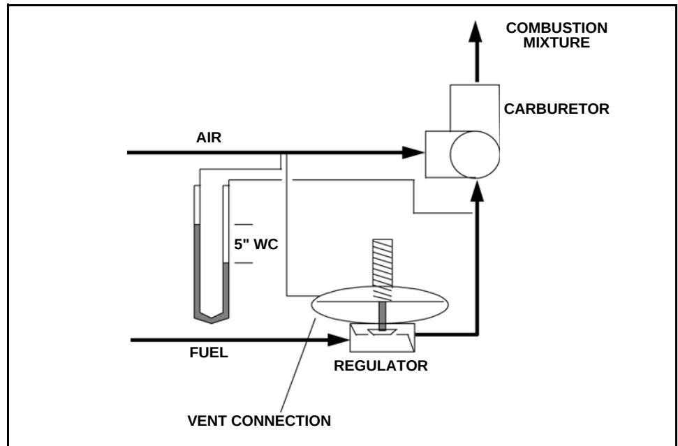
Figure 8-11 Engine Fuel Regulator
