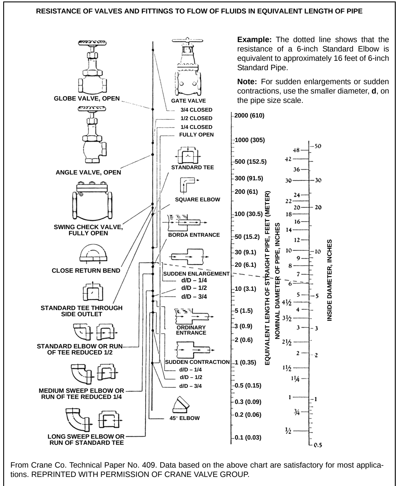
Figure 4-11 Equivalent Pipe Length Of Fittings In Feet (meters)
