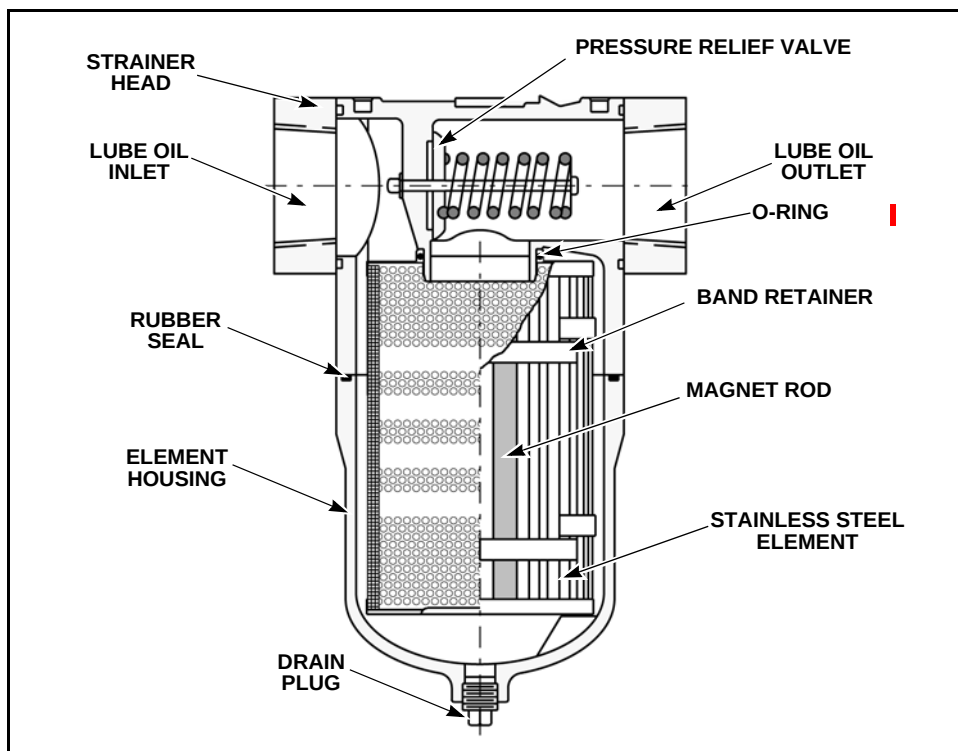
Figure 5-5 Lube Oil Strainer
