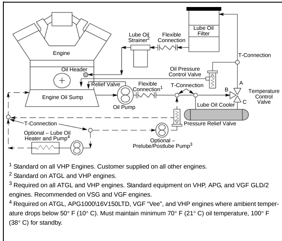
Figure 5-1 General Piping Schematic
