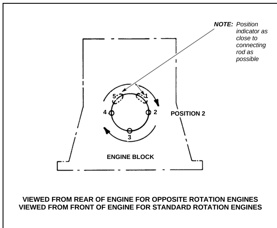
Figure 2-15 Locations For Checking Crankshaft Deflection
