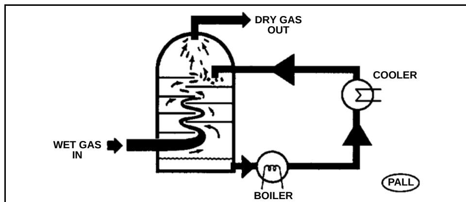
Figure 8-14 Absorption Deliquescent Dryer (Liquid)
