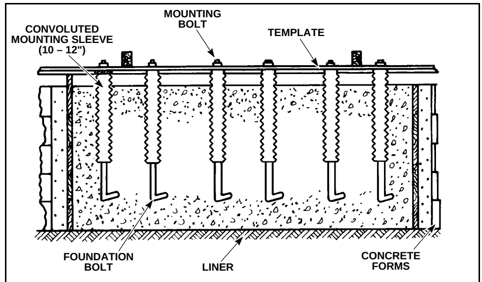
Figure 1-10 Mounting Sleeves Embedded in Concrete
