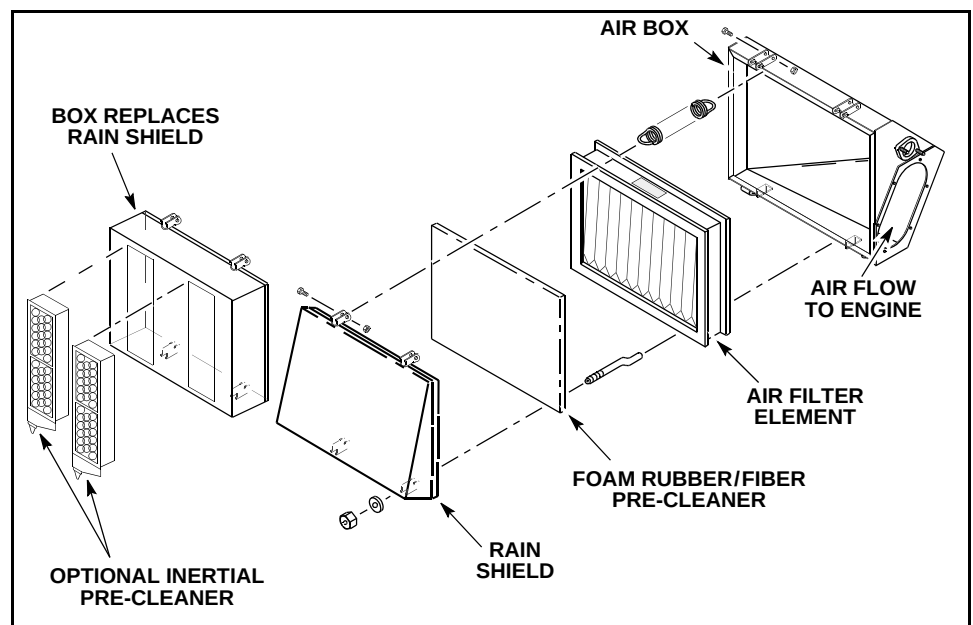
Figure 6-3 Typical Air Cleaner Components
