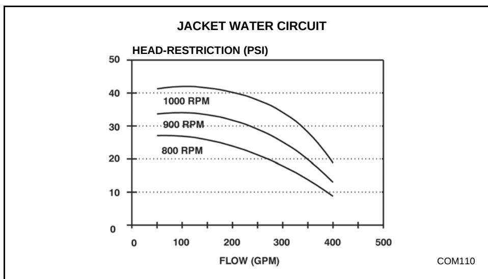
Figure 4-5 Water Pump Output
