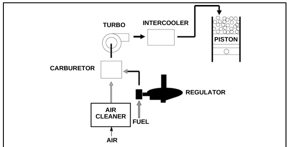
Figure 8-3 GSID Rich Burn Turbocharged Draw-Thru Fuel System
