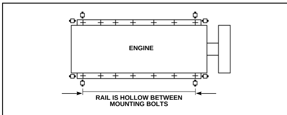
Figure 9-6 Horizontal Jacking
