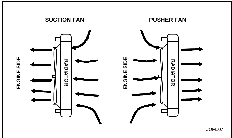
Figure 4-2 Suction and Pusher Fans
