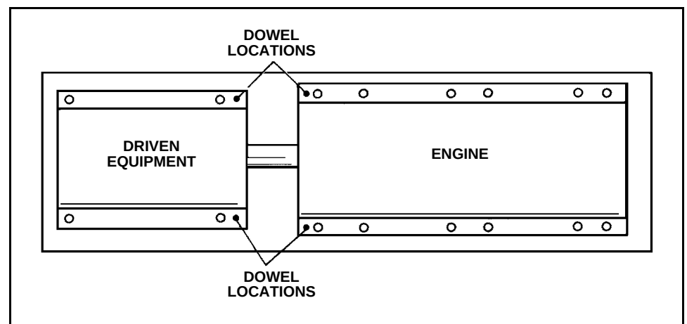
Figure 2-46 Dowel Placement
