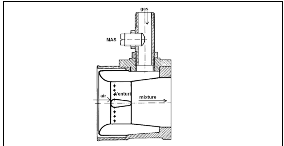
Figure 8-6 Venturi Type Carburetor
