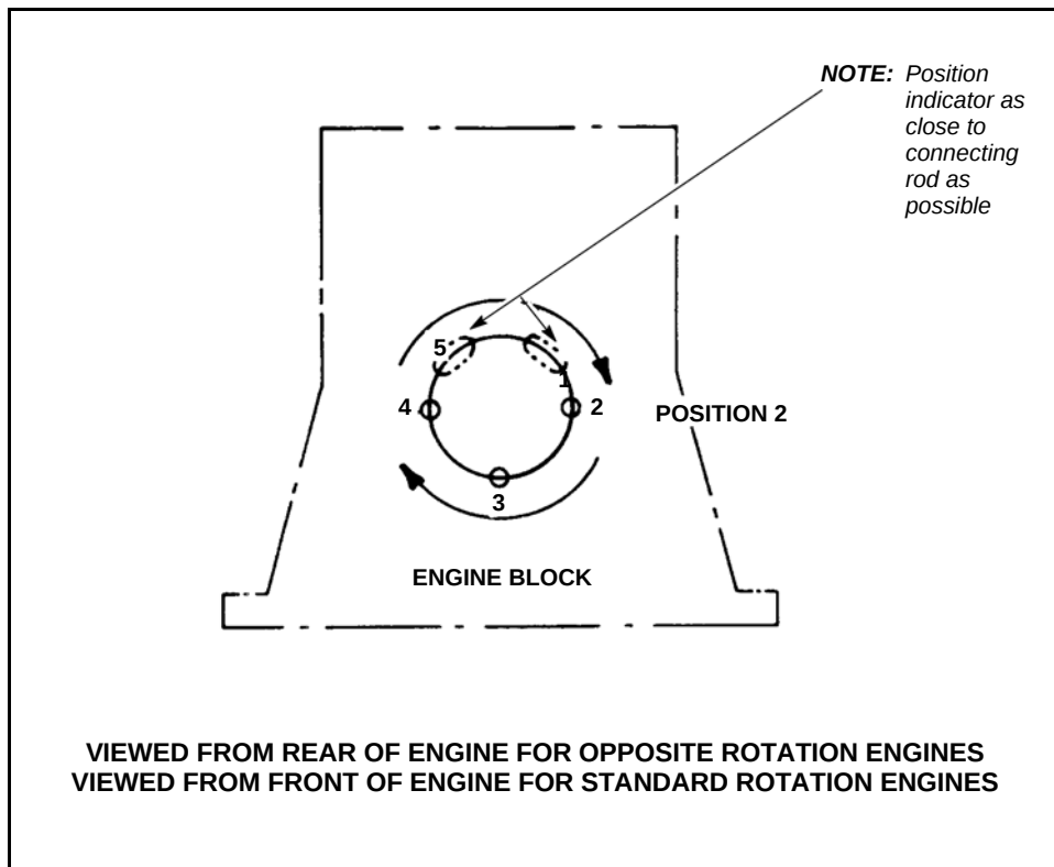
Figure 2-22 Location For Checking Crankshaft Deflection
