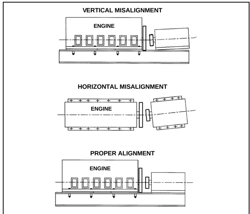
Figure 9-6 Angular Alignment
