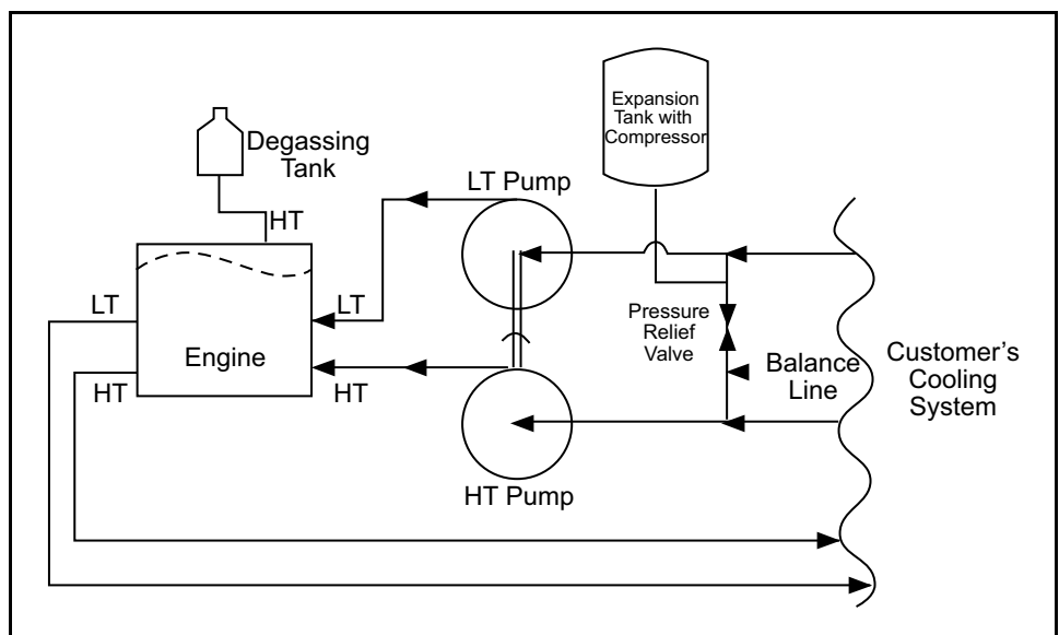
Figure 4-15 APG Bladder Style Pressurization System With Degassing Tank
