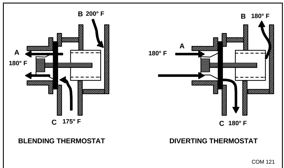
Figure 4-18 Blending and Diverting Thermostats
