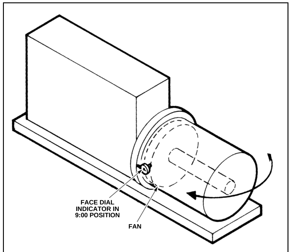
Figure 2-30 Dial Indicator Positioning
