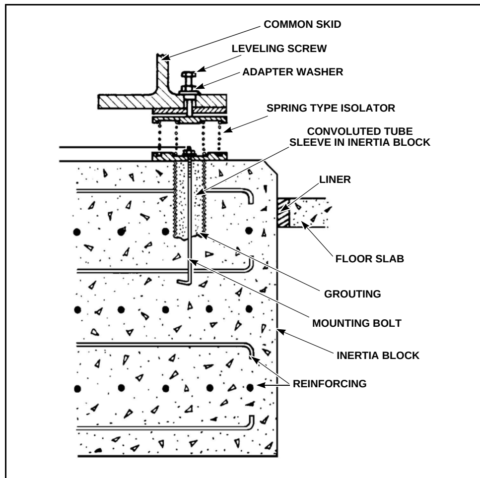
Figure 1-6 Schematic Spring Isolator Mounting Pad Construction
