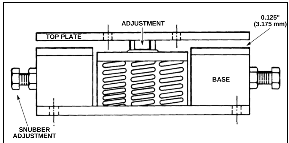
Figure 2-16 Spring Isolator Mount
