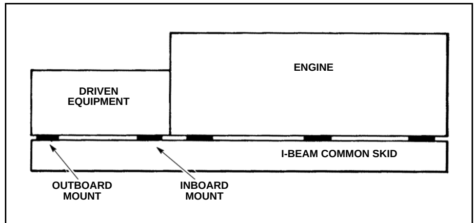
Figure 2-29 Add Or Remove Shims From The Mounts On Each End Of The Machine To Make Vertical Adjustments
