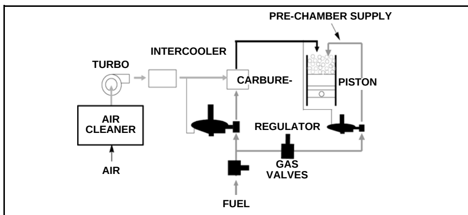
Figure 8-4 Pre-Chamber Lean Combustion Engine (Blow-Thru)
