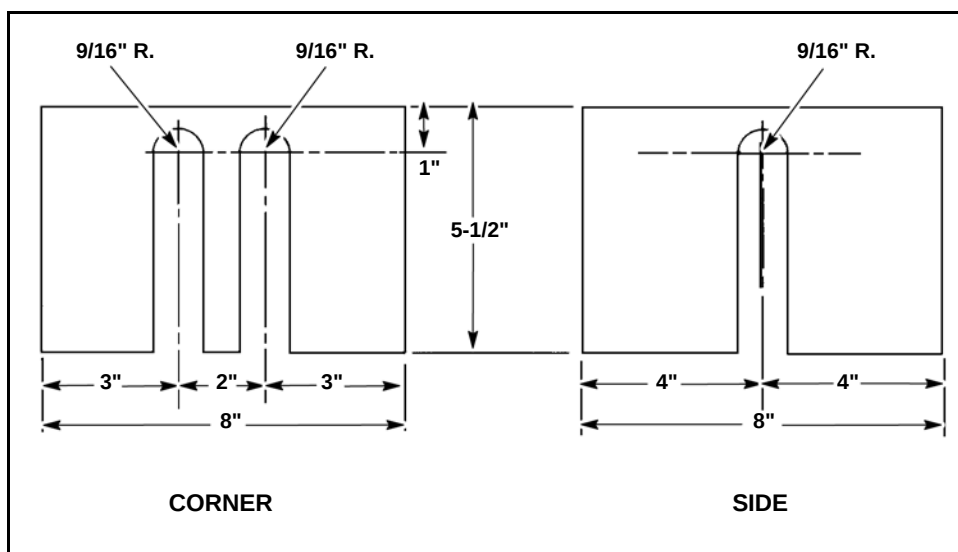
Figure 2-4 Shim Specifications
