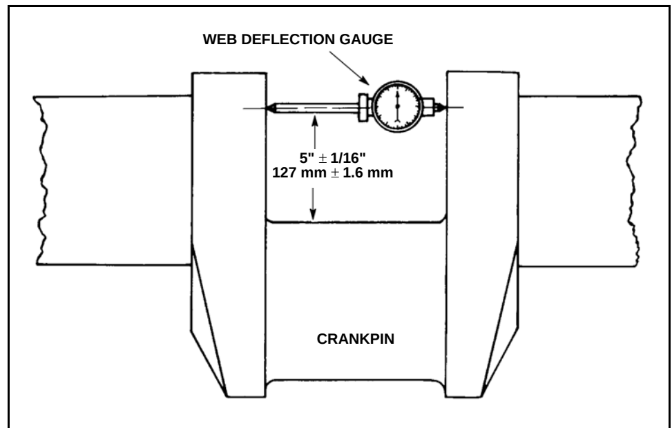
Figure 2-21 Crankshaft Web Deflection
