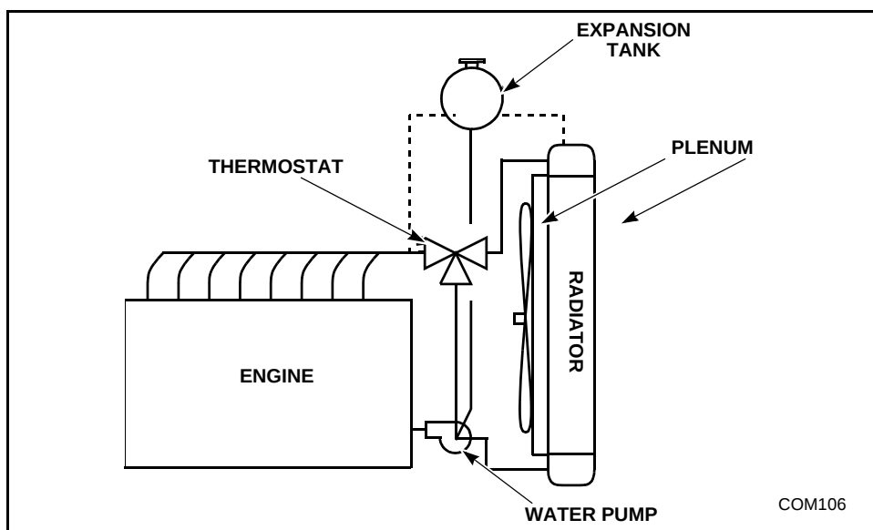
Figure 4-1 Schematic of Engine and Radiator
