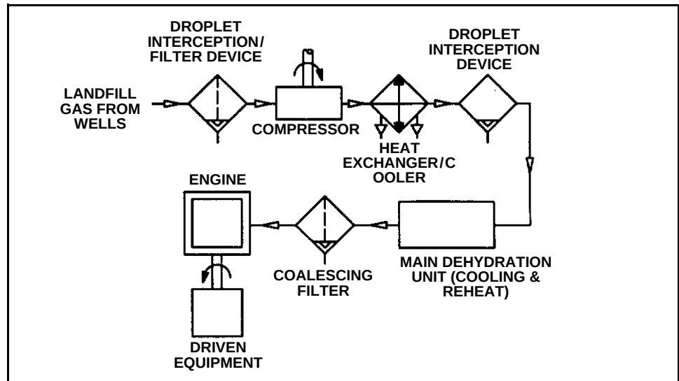
Figure 8-16 Typical Landfill Gas Fuel Treatment System
