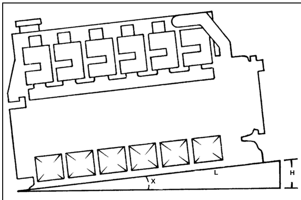
Figure 1-15 Determine Angle of Operation
