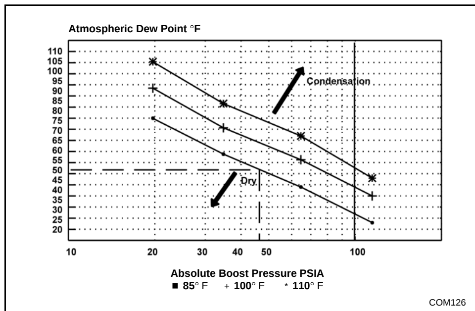
Figure 4-25 Boost Pressure vs. Dew Point To Determine Intake Manifold Condensation
