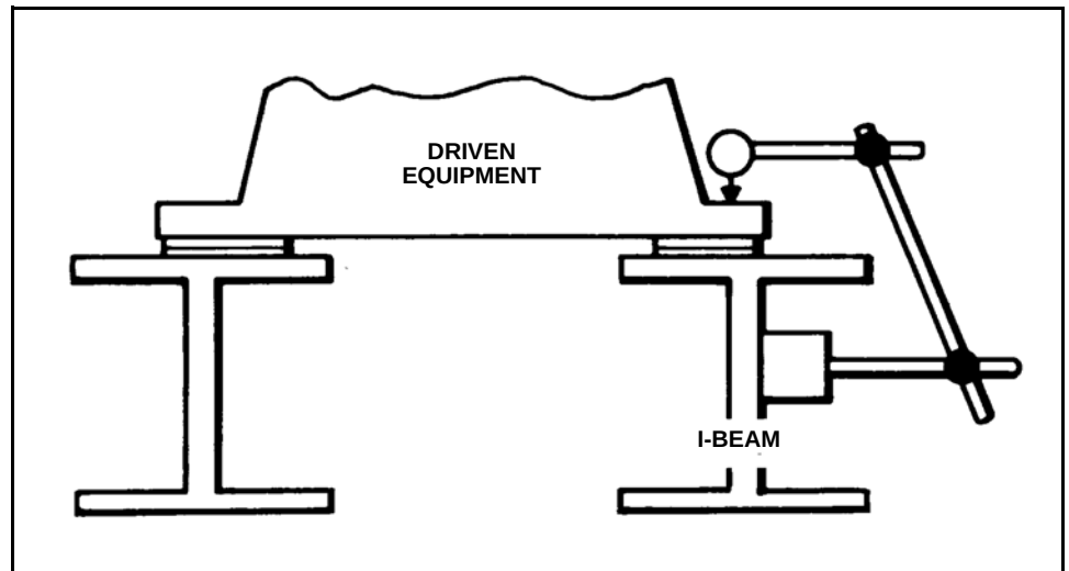
Figure 2-23 Driven Equipment Base Deflection
