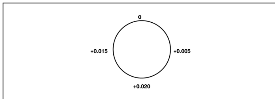
Figure 9-18 Total Indicator Reading (TIR)
