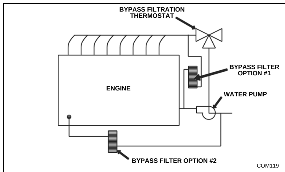
Figure 4-16 Schematic for Bypass Water Filtration Systems
