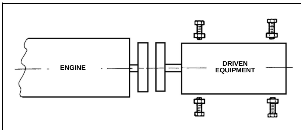
Figure 2-42 Correct Angular Alignment
