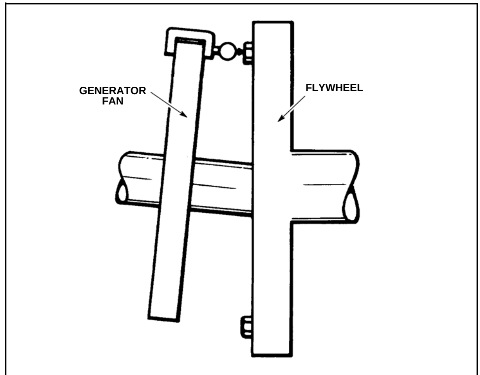
Figure 2-25 Angular Alignment-Single Bearing Generator
