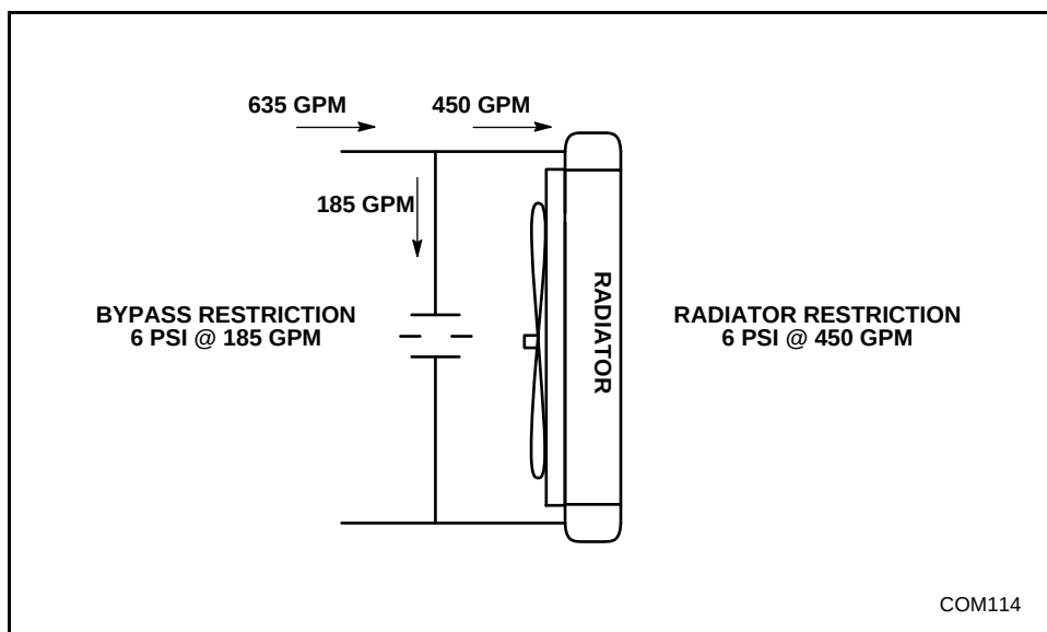
Figure 4-9 Cooling System with Bypass Pipe
