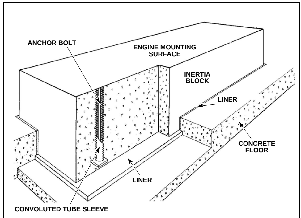
Figure 1-5 Cross Section of Concrete Inertia Block
