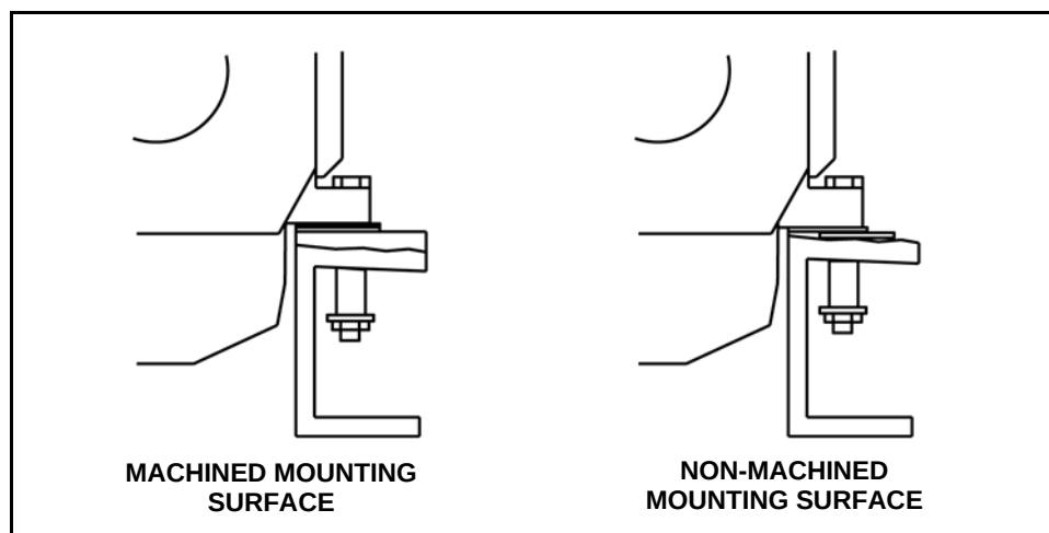
Figure 9-1 Machined Surface Mounting
