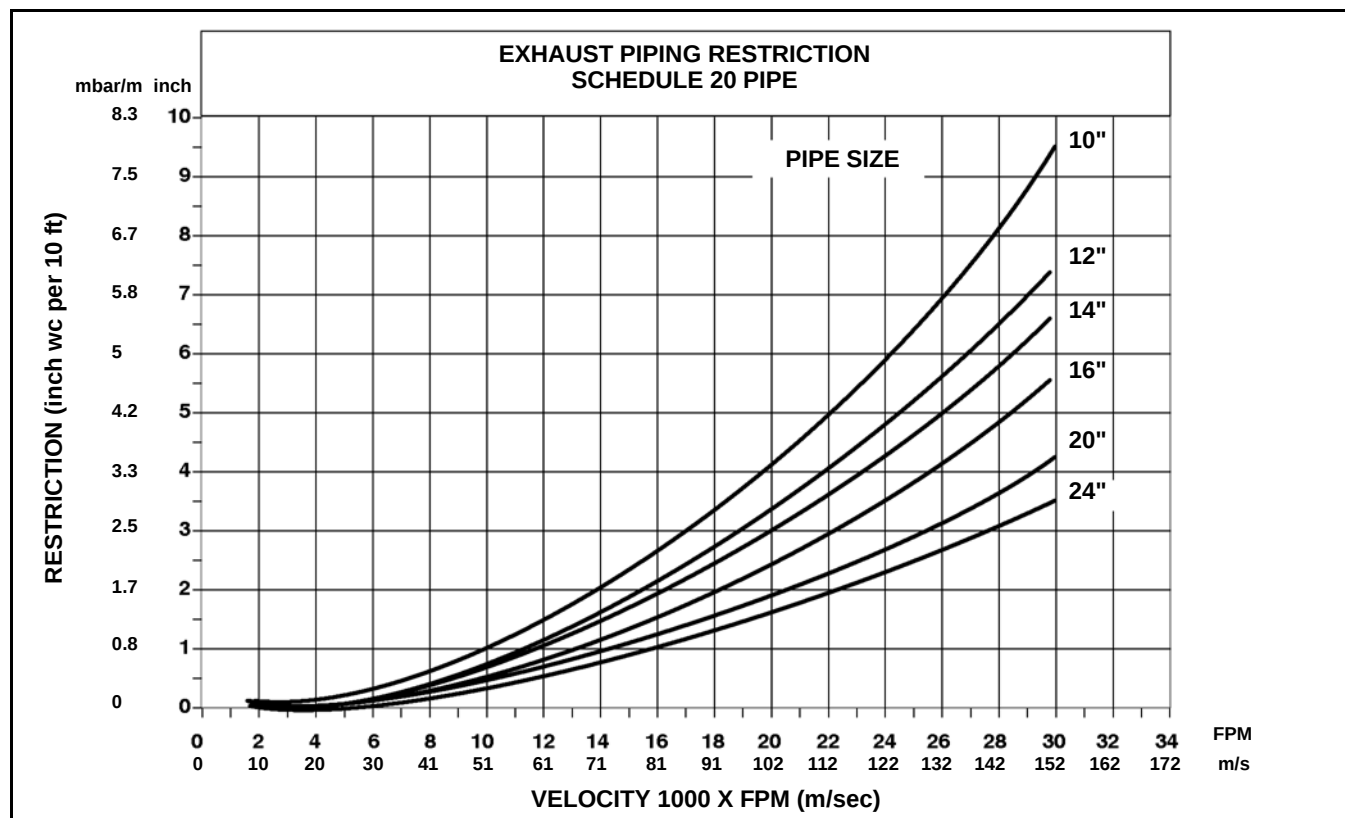
Figure 7-4 Restriction Vs. Velocity for Pipe Diameter up to 24"
