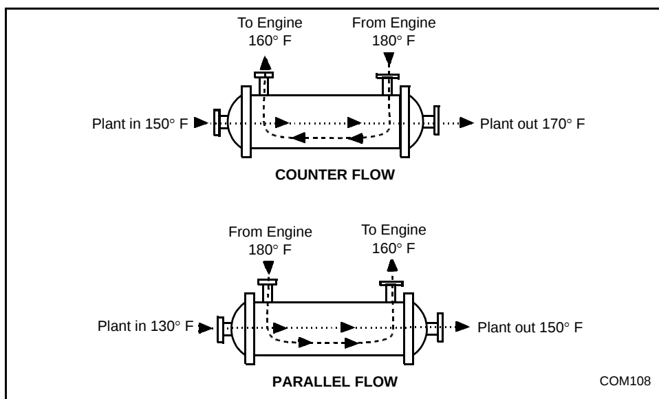
Figure 4-3 Counter and Parallel Flow Heat Exchanger
