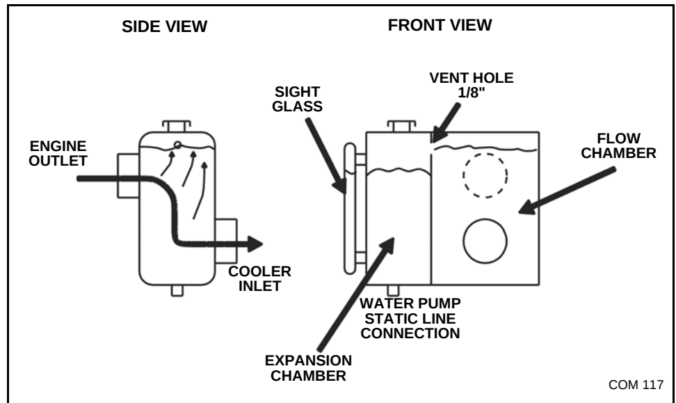
Figure 4-13 Surge Tank
