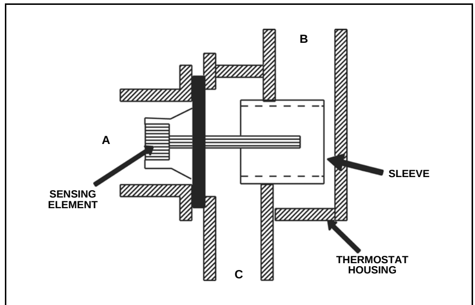
Figure 4-17 Thermostat
