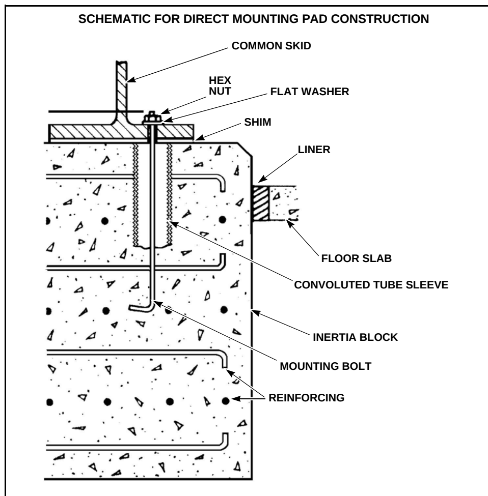
Figure 1-4 Common Skid Mounted Directly to Inertia Block or Pad
