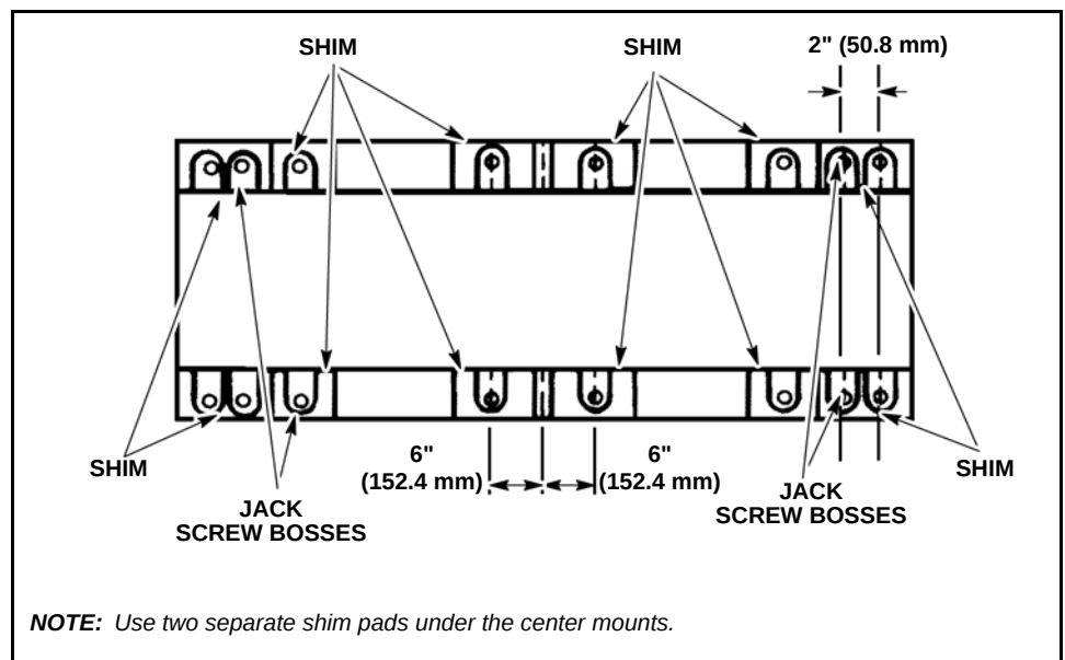
Figure 2-3 Engine Shimming Procedure
