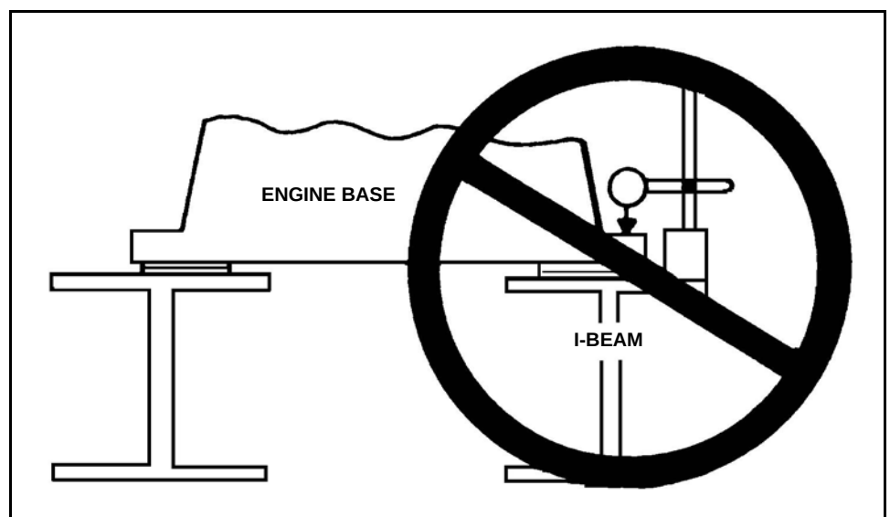
Figure 2-6 Incorrect Mounting
