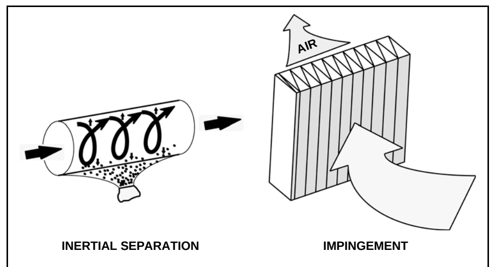
Figure 6-1 Air Filtration By Inertial Separation And Impingement
