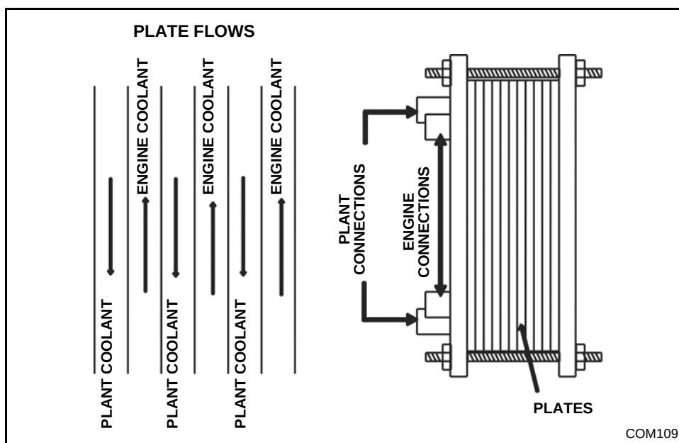
Figure 4-4 Plate-Type Heat Exchanger
