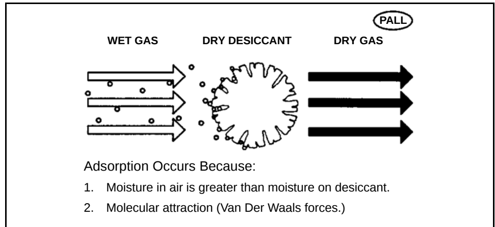
Figure 8-15 Adsorption Drying
