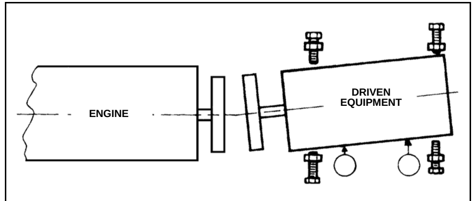
Figure 2-39 Indicator Positioning
