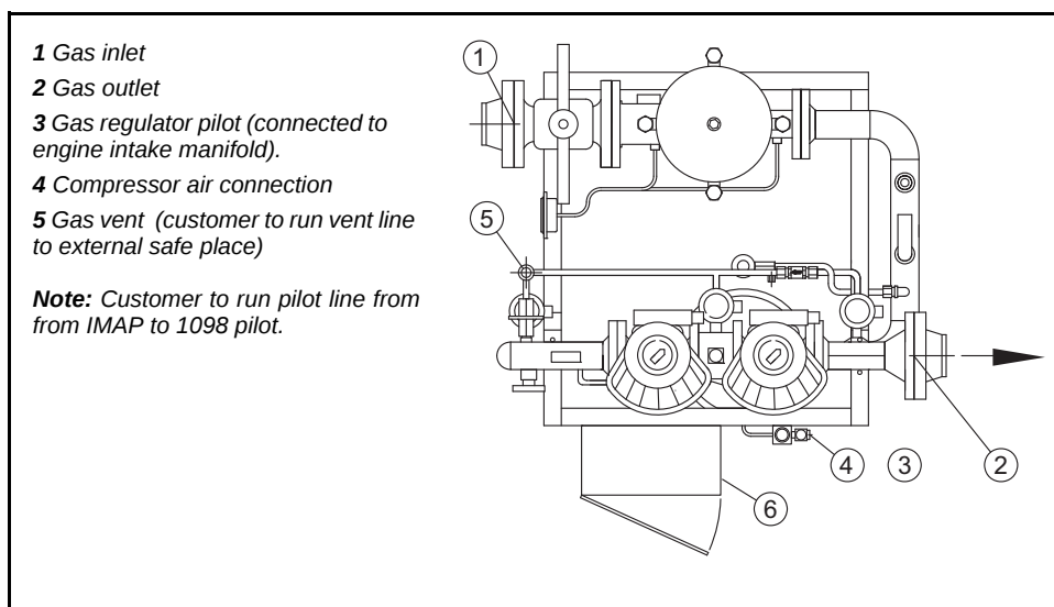
Figure 8-12 APG2000/APG3000 Gas Train
