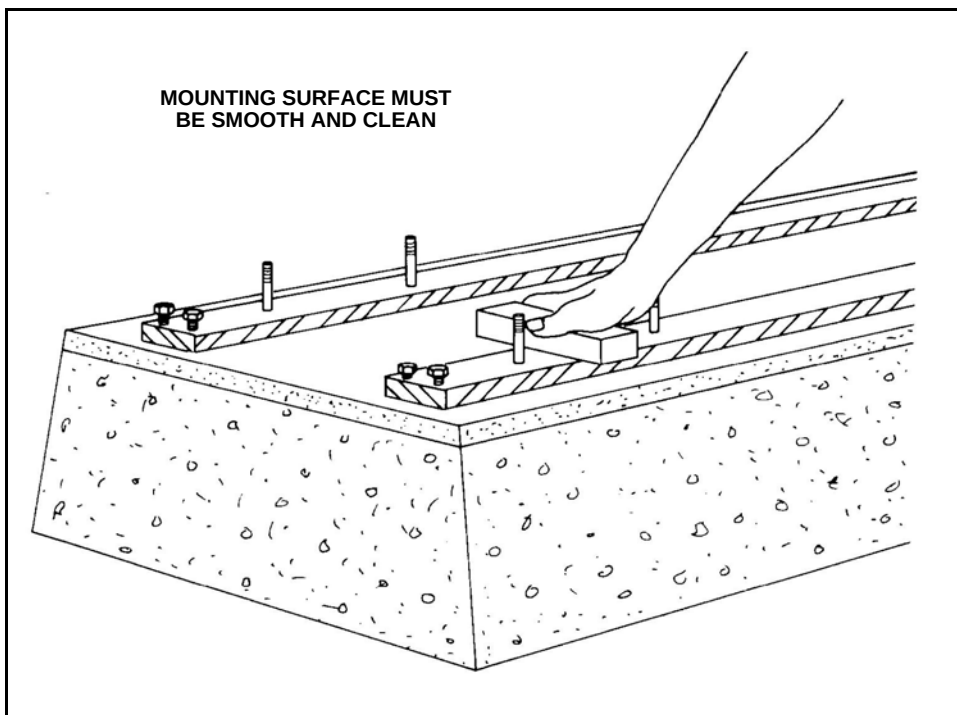
Figure 2-2 Mounting Pad
