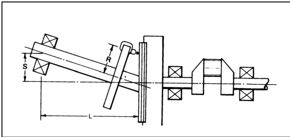
Figure 2-28 Exaggerated Example
