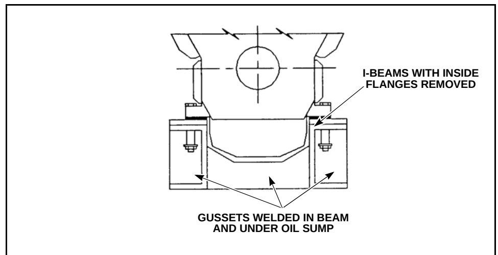
Figure 9-8 Engine Mounted Directly Above Web
