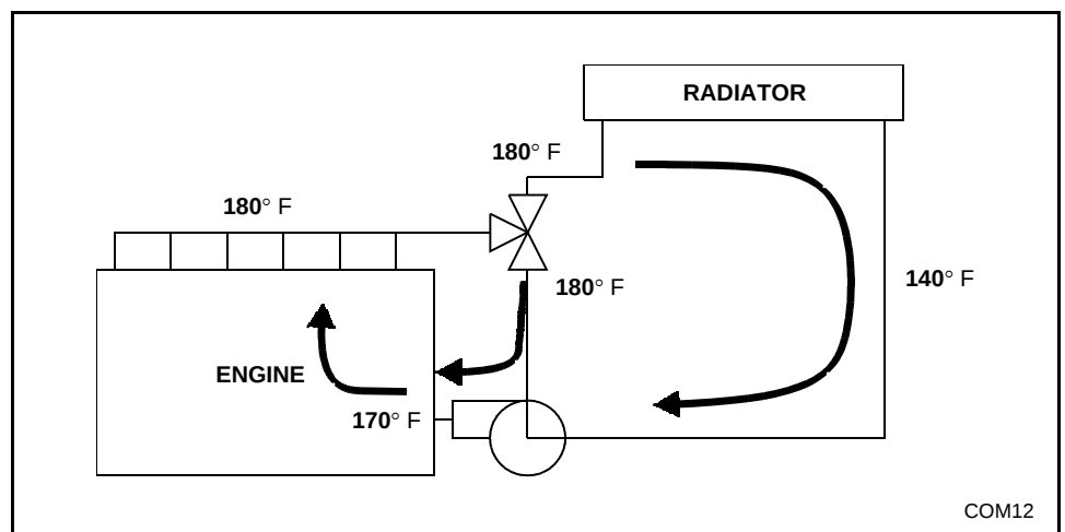
Figure 4-21 Thermostat Partially Open
