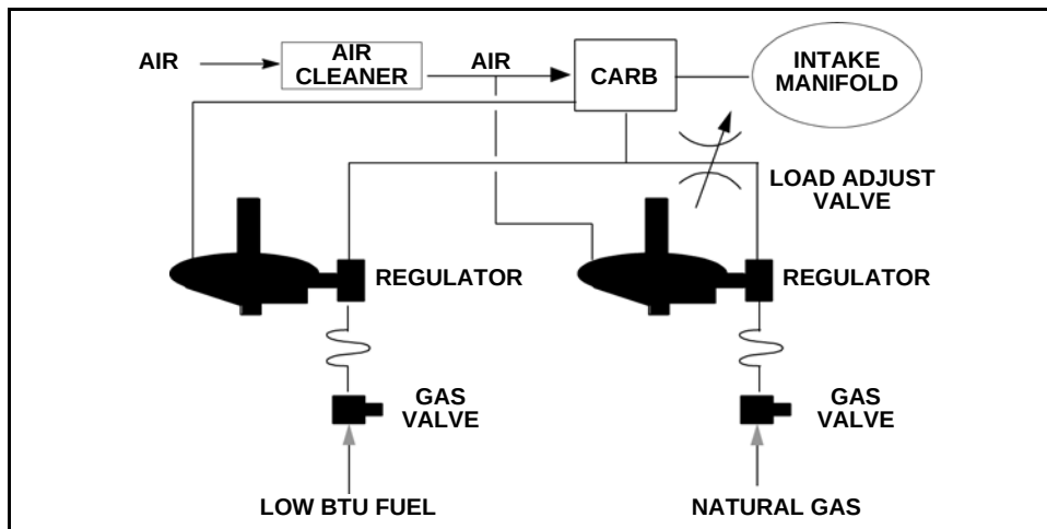
Figure 8-8 Single Carburetor
