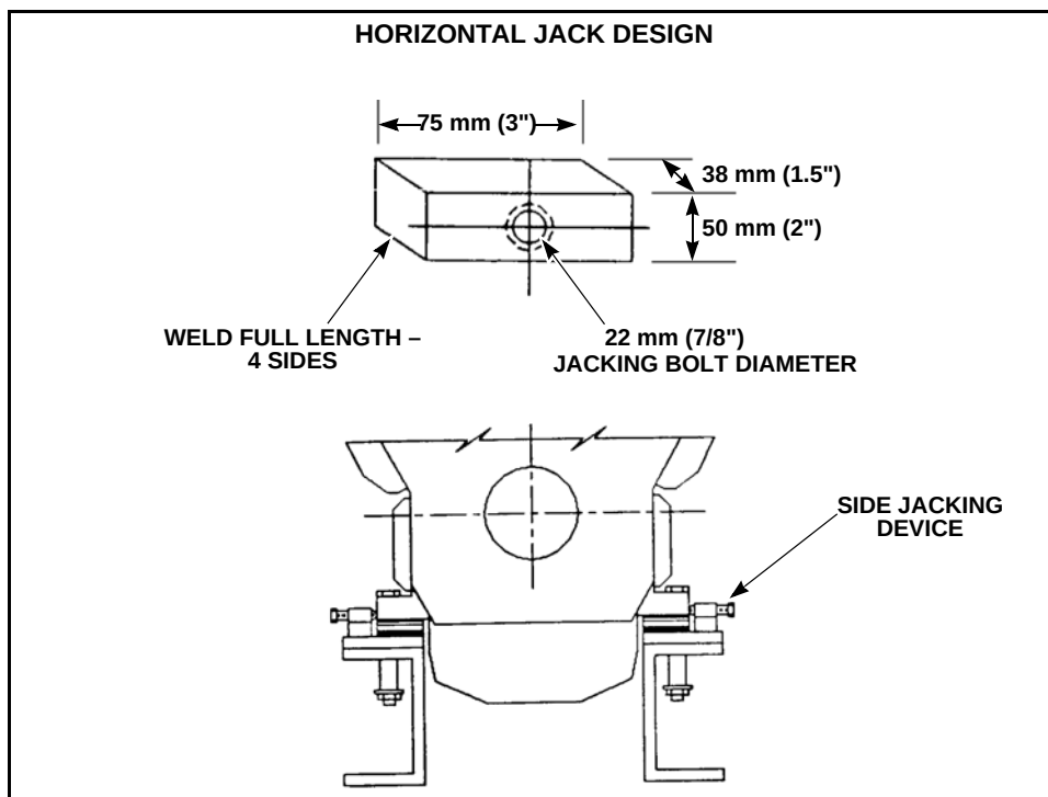
Figure 9-7 Jacking Devices
