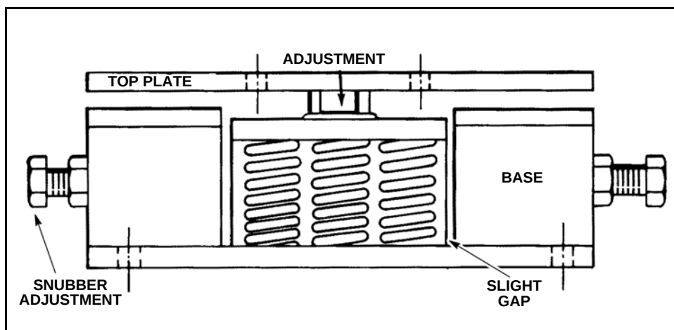
Figure 2-18 Spring Isolator Mount
