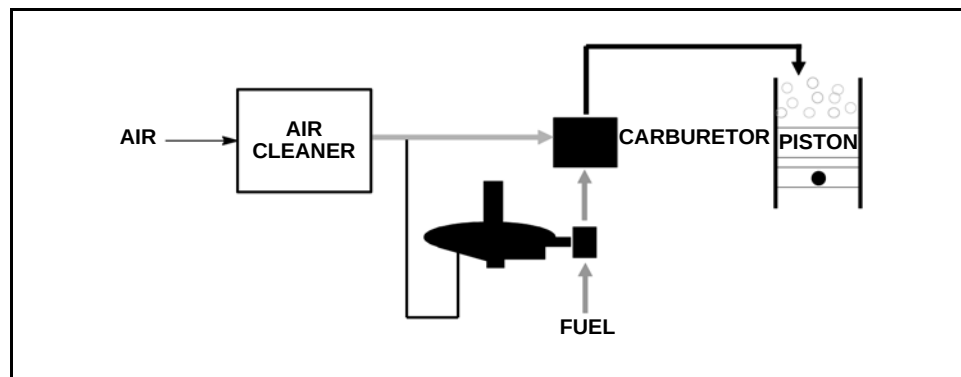
Figure 8-1 Naturally Aspirated Engine
