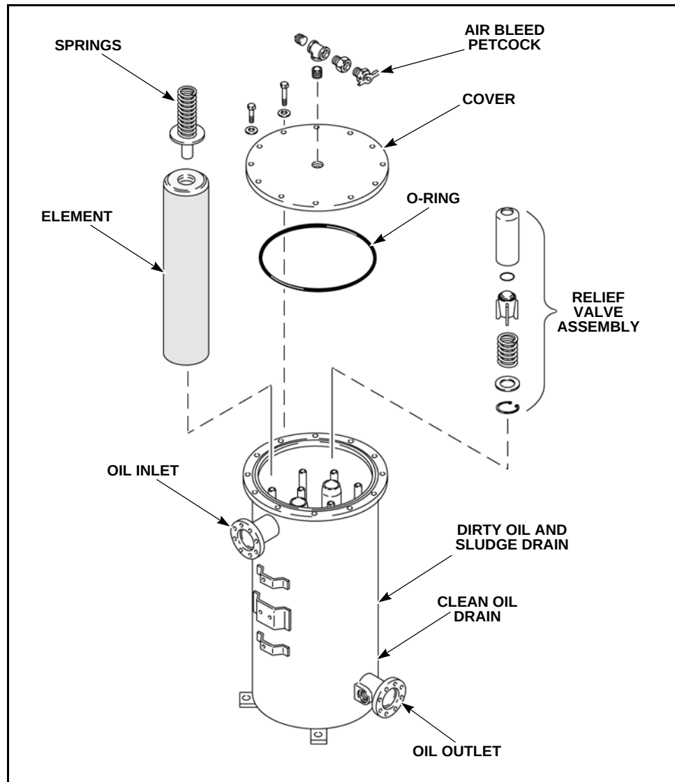
Figure 5-2 Full-Flow Lube Oil Filter (VHP Canister Type)
