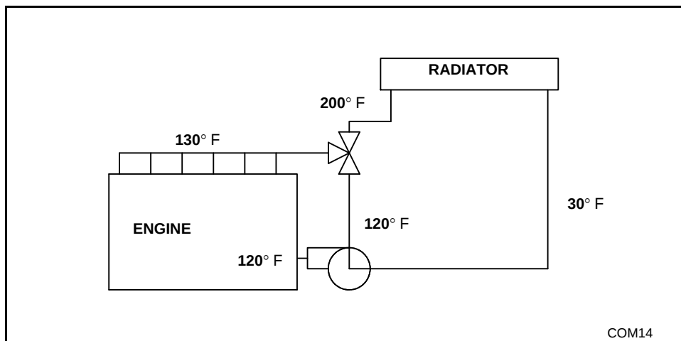
Figure 4-23 Thermostat Fully Closed
