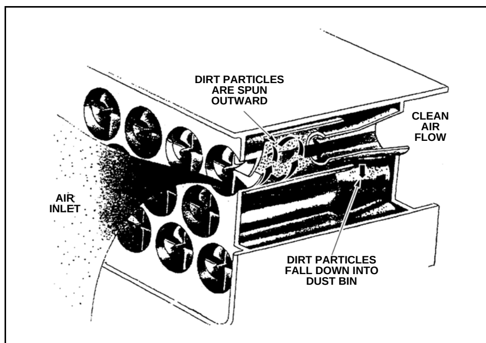
Figure 6-2 Inertial Type Precleaner
