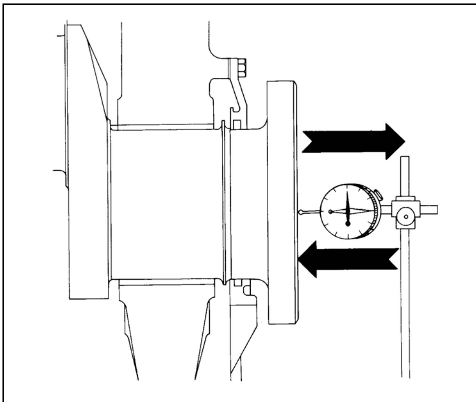
Figure 2-31 Checking Crankshaft End Play
