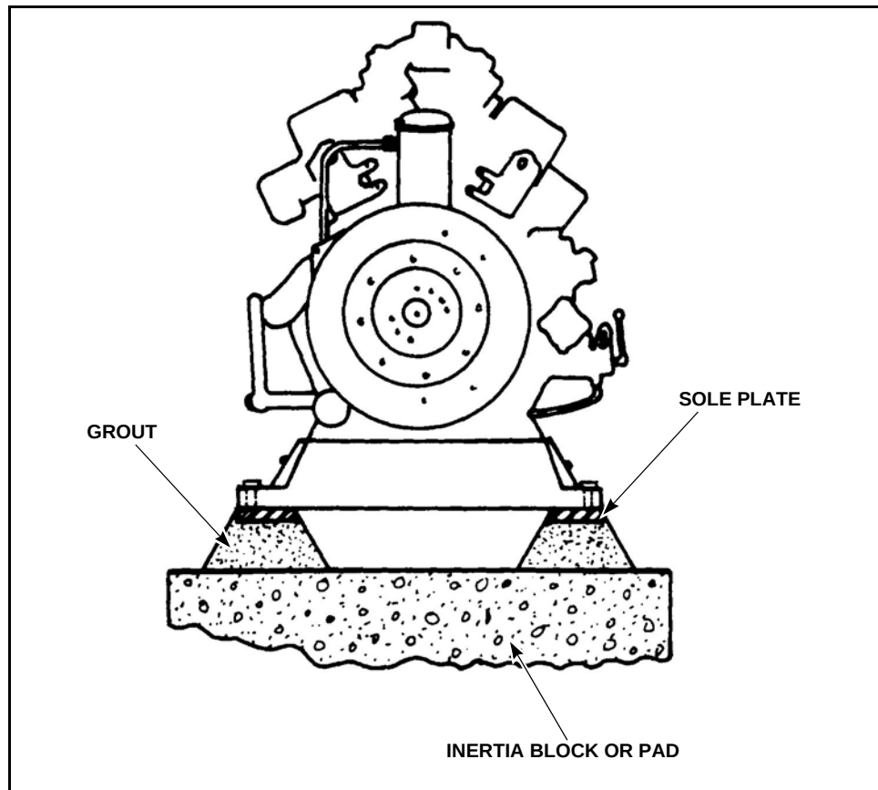
Figure 1-13 Rear View of Mounted Engine
