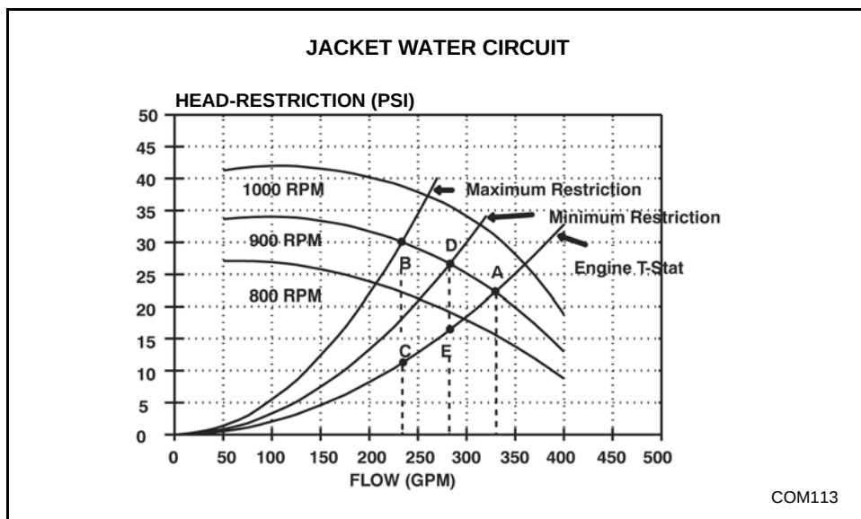
Figure 4-8 Water Pump Curve with Minimum Restriction
