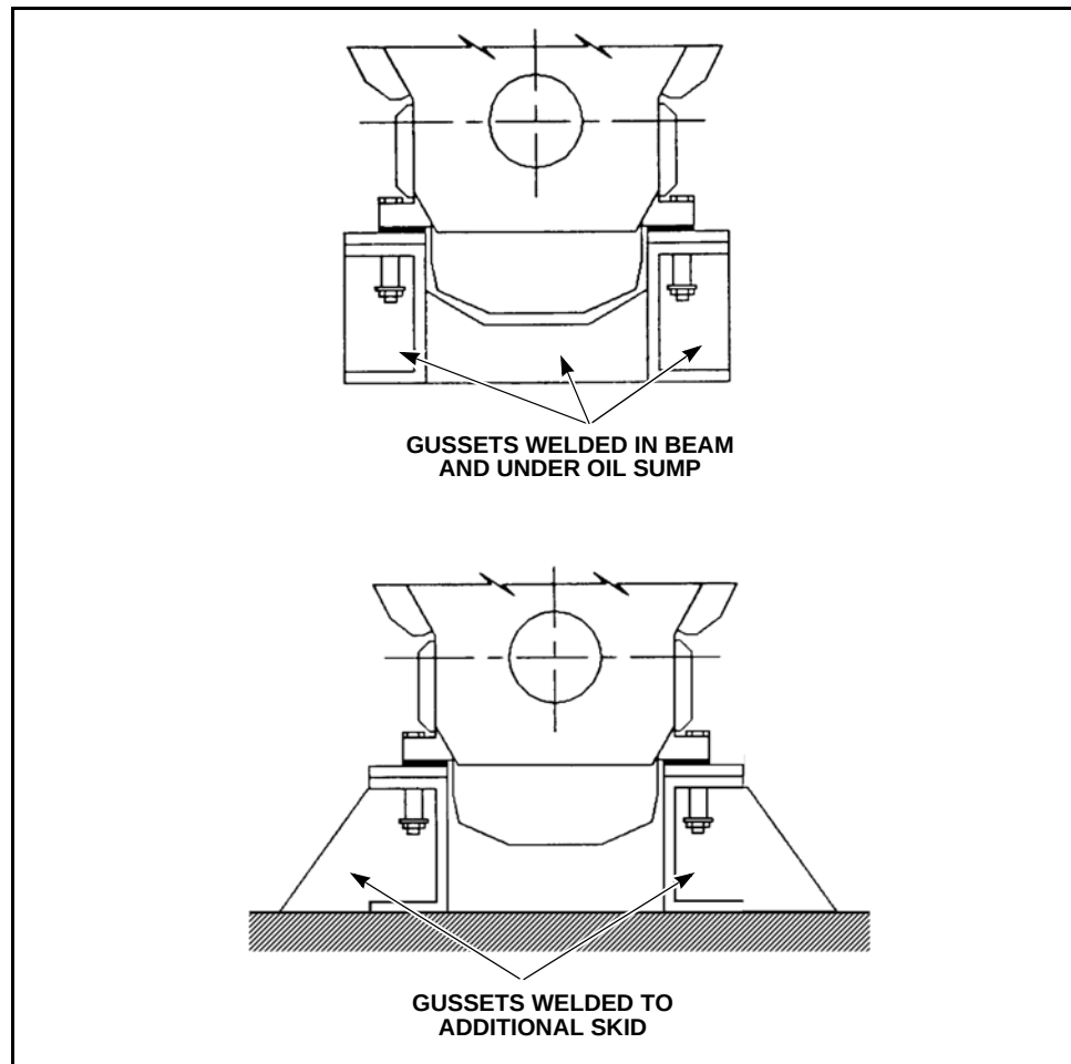
Figure 9-9 Additional Gussets Added
