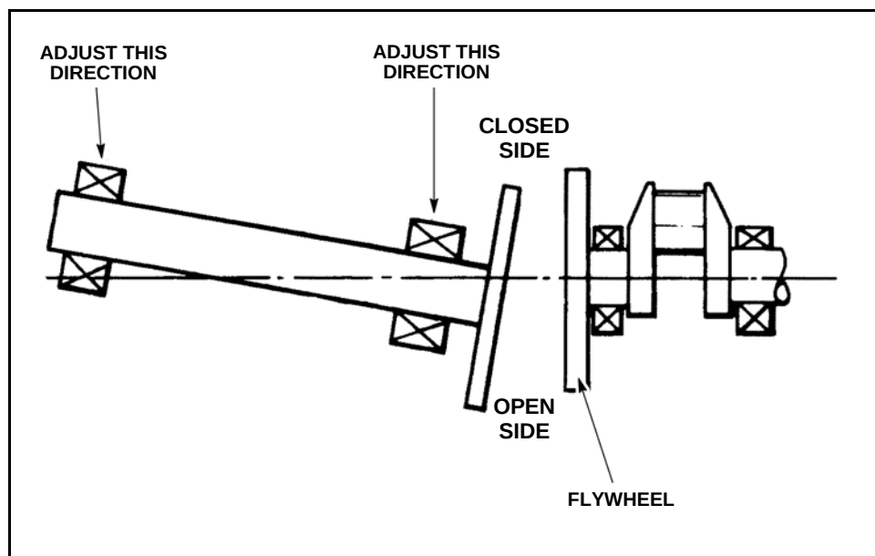
Figure 2-38 Make Adjustment To Close The Open Side Of The Coupling
