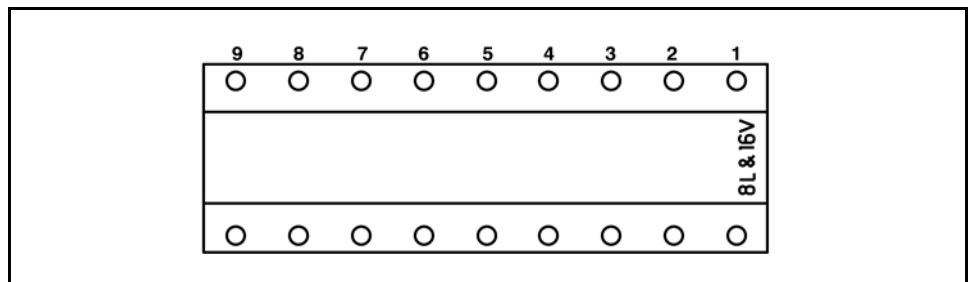
Figure 9-3 Bolt Locations for 8 and 16 Cylinder Models
