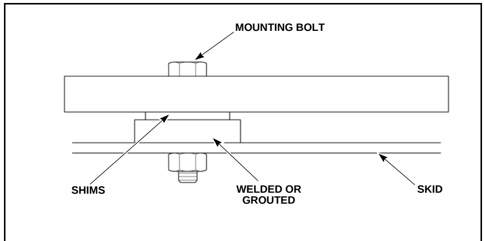
Figure 9-2 Shimming an Engine
