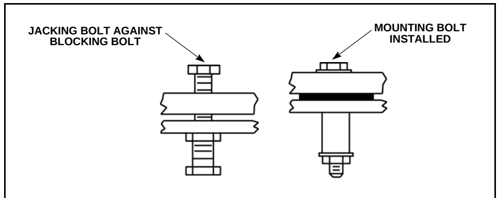
Figure 9-5 Jacking Using Mounting Bolt
