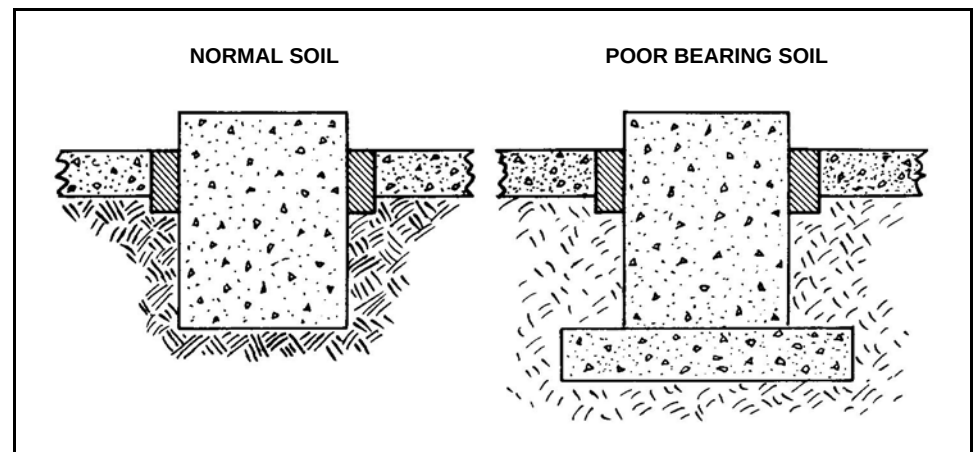
Figure 1-3 Footing for Poor Bearing Soil
