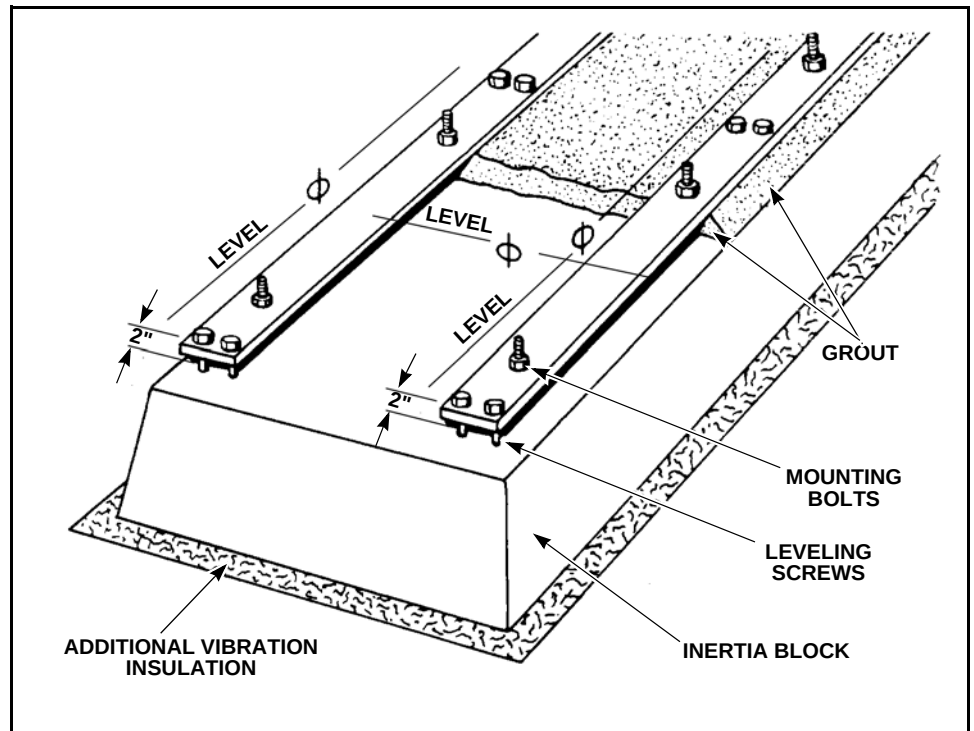
Figure 1-12 Grouting the Inertia Block
