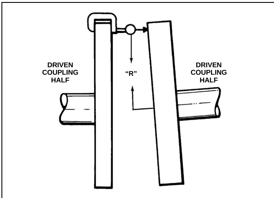
Figure 2-34 Measuring Angular Alignment
