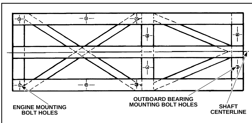
Figure 1-9 Template
