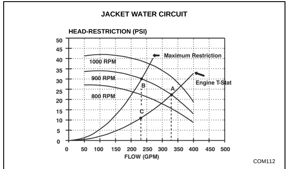
Figure 4-7 Water Pump Curve with Maximum Restriction
