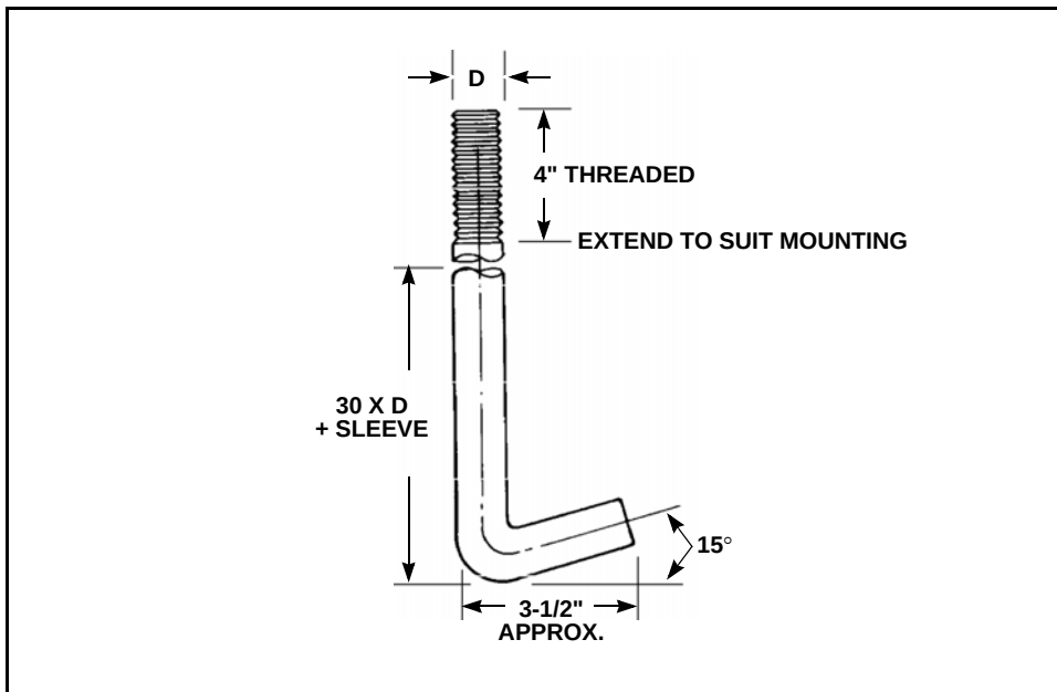
Figure 1-8 Mounting Bolt
