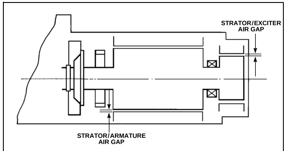
Figure 2-32 Single Bearing Generator
