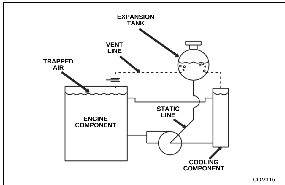
Figure 4-12 Schematic of Cooling Circuit
