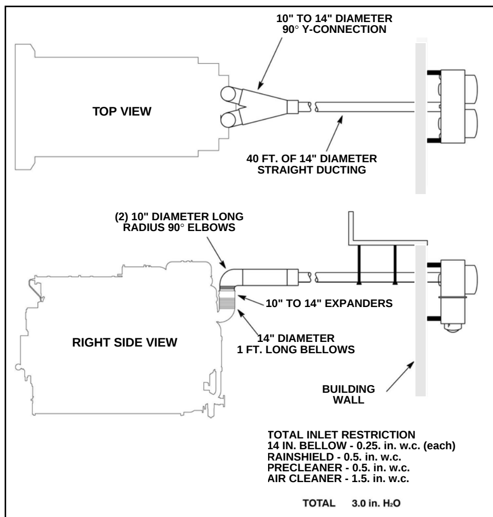
Figure 6-4 Proposed Air Induction System
