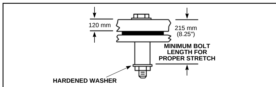
Figure 9-3 Hardened Washer
