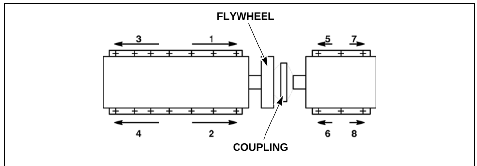
Figure 9-4 Belt Tightening Pattern
