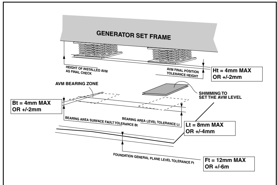
Figure 1-14 Mounting AVMs (Anti Vibrating Mounts)
