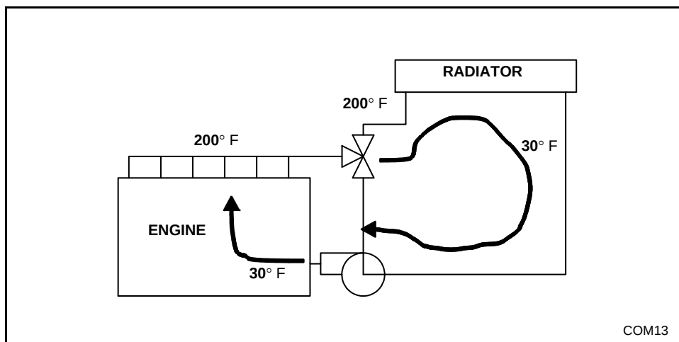
Figure 4-22 Thermostat Fully Open
