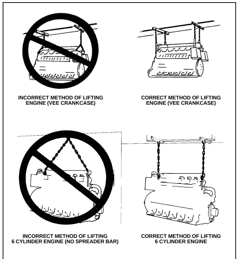
Figure 2-1 Engine Lifting Procedures
