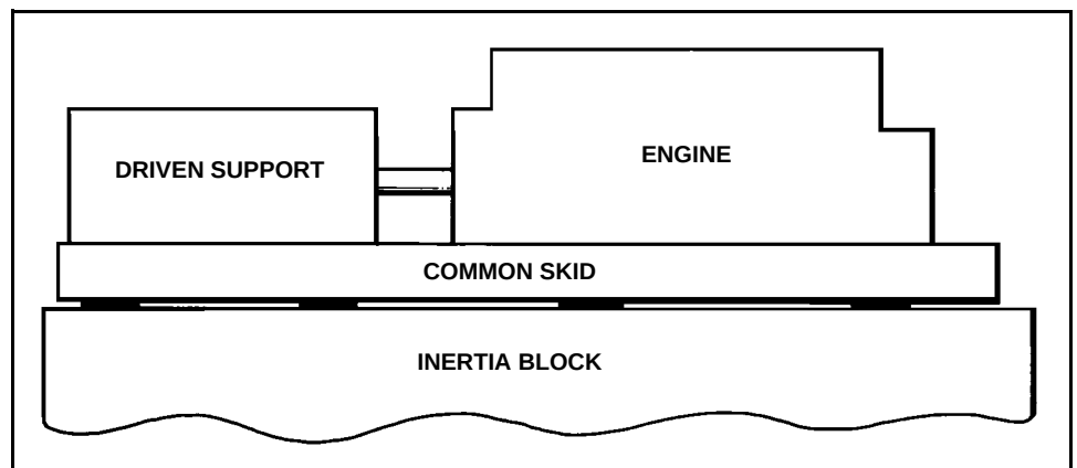
Figure 1-1 Engine and Driven Equipment on Common Skid
