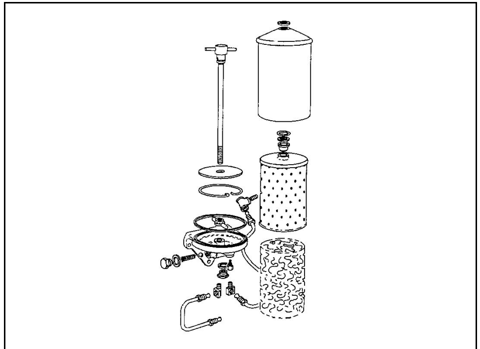
Figure 5-3 Oil Filter – Shunt Type
