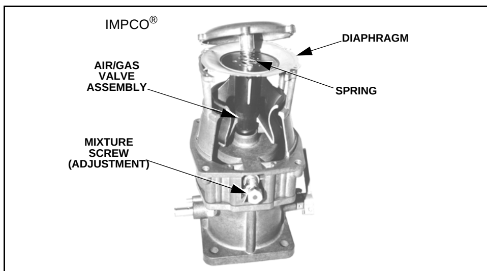
Figure 8-7 IMPCO® Carburetor
