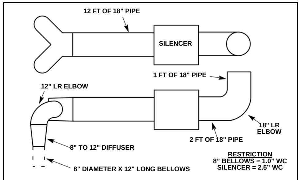
Figure 7-6 Schematic for Sample Problem
