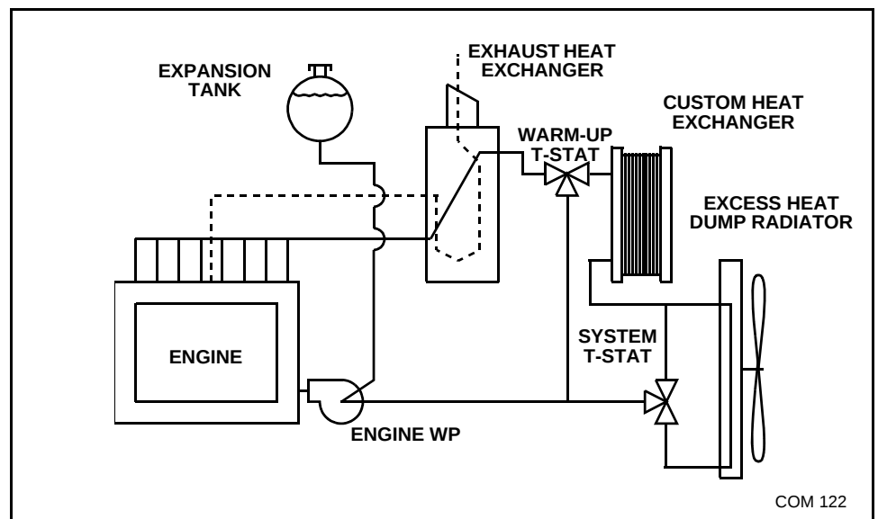
Figure 4-19 Single Pump Heat Recovery System (vent lines not pictured)
