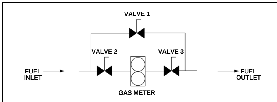
Figure 8-19 Gas Meter Bypass Piping
