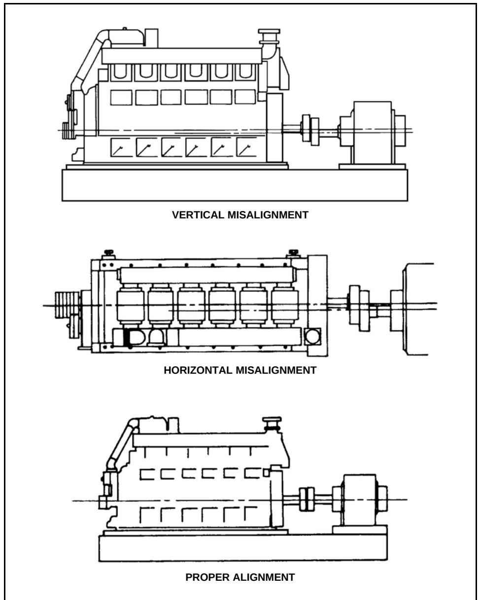
Figure 2-45 Parallel Alignment
