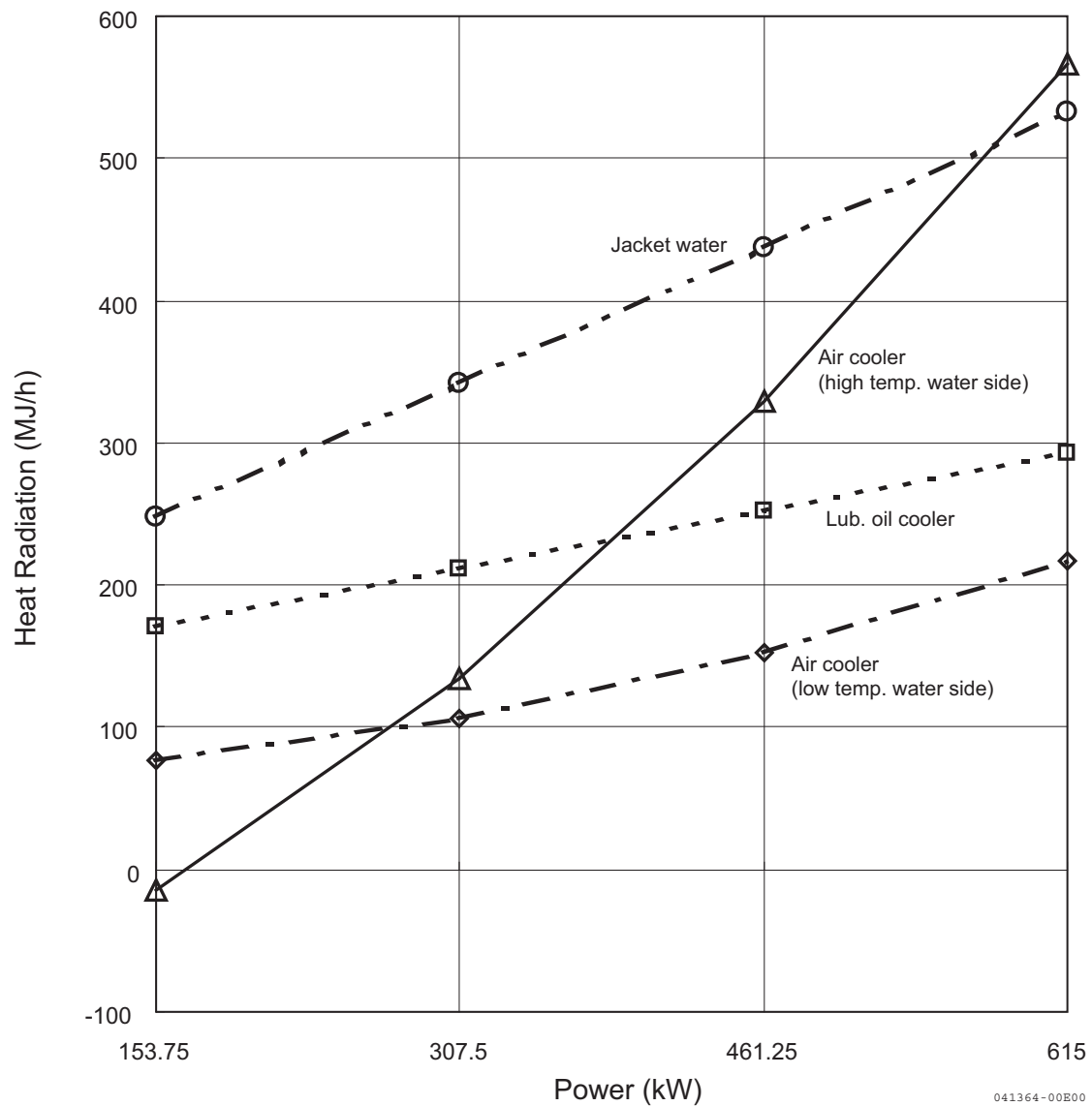
Heat Radiation
