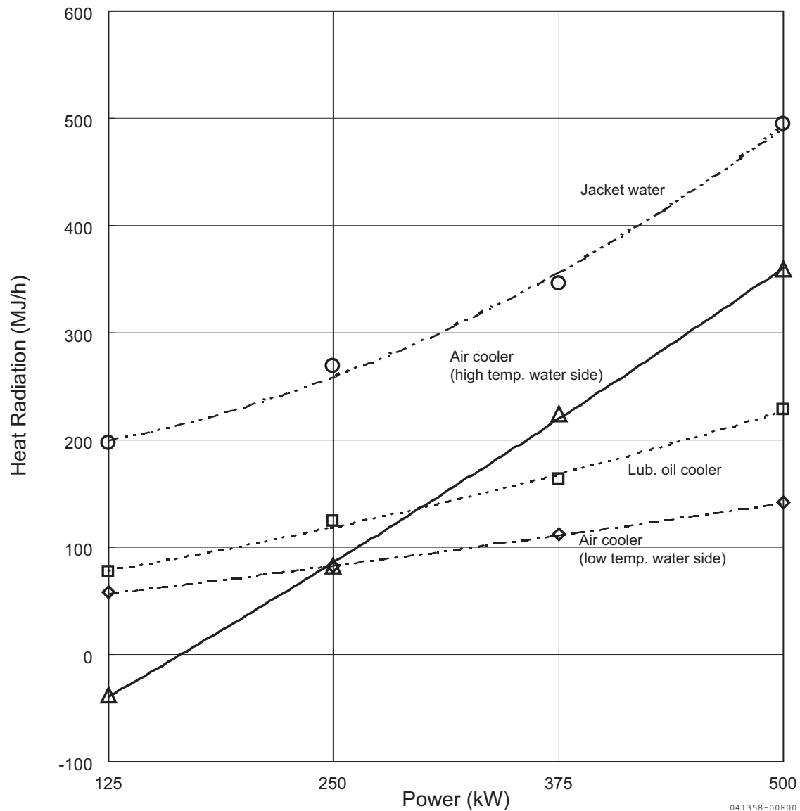
Heat Radiation
