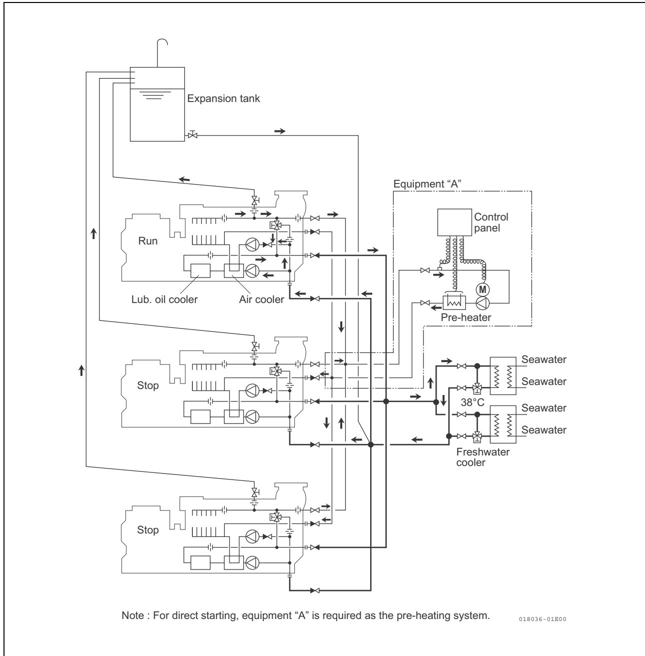
Fig.(b) Pre-Heating System with Pre-Heater
