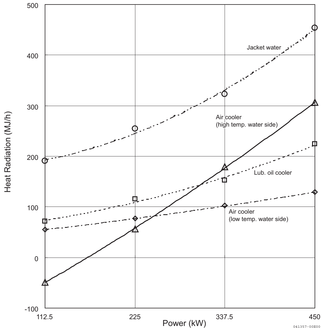
Heat Radiation
