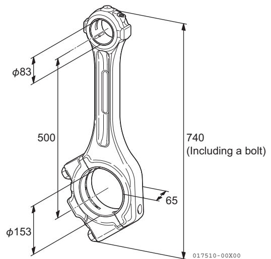
Connecting Rod
