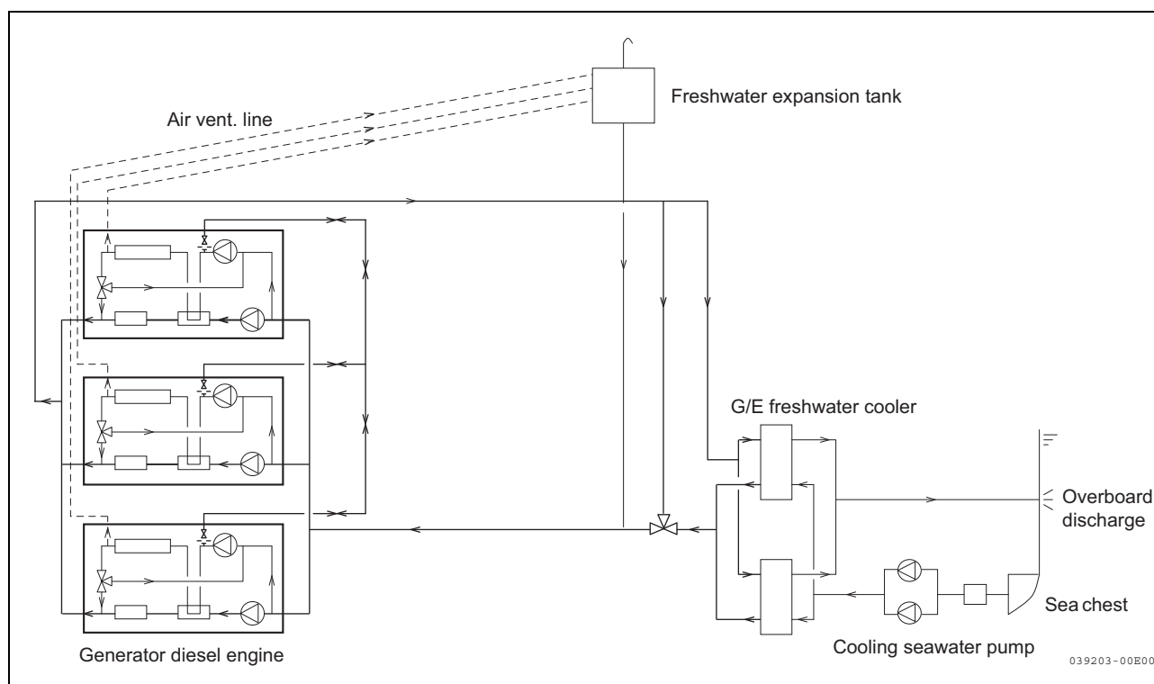
Fig.(a) Mutual Engine Warming Up System
