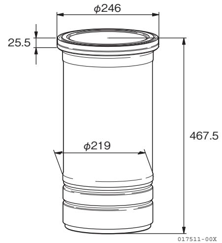
Cylinder Liner
