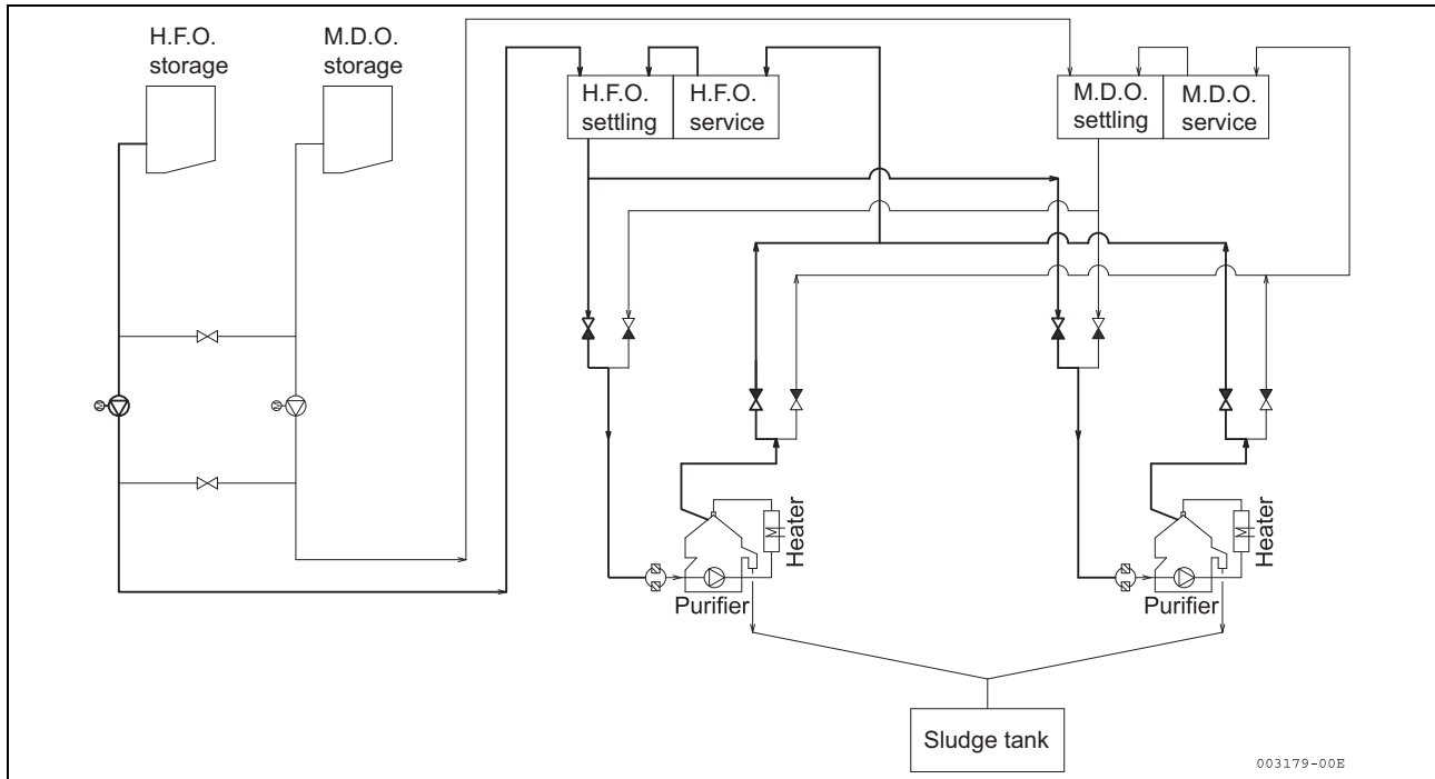
Fuel Pre-Treatment System Diagram (Reference)
