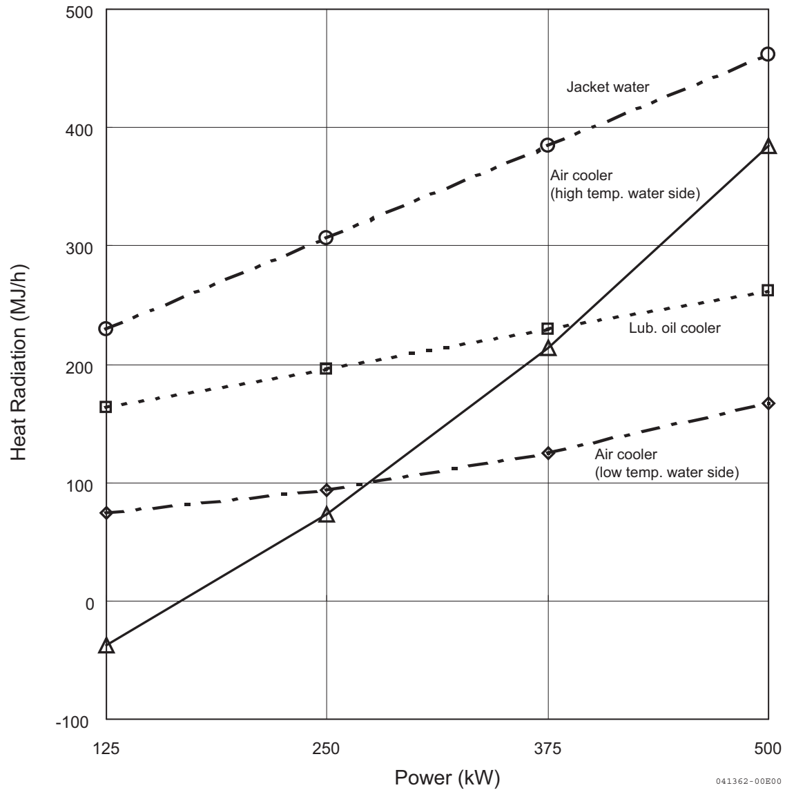
Heat Radiation
