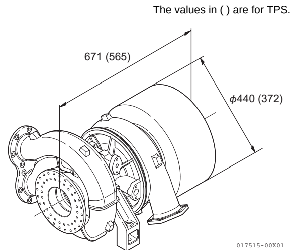
Turbocharger
