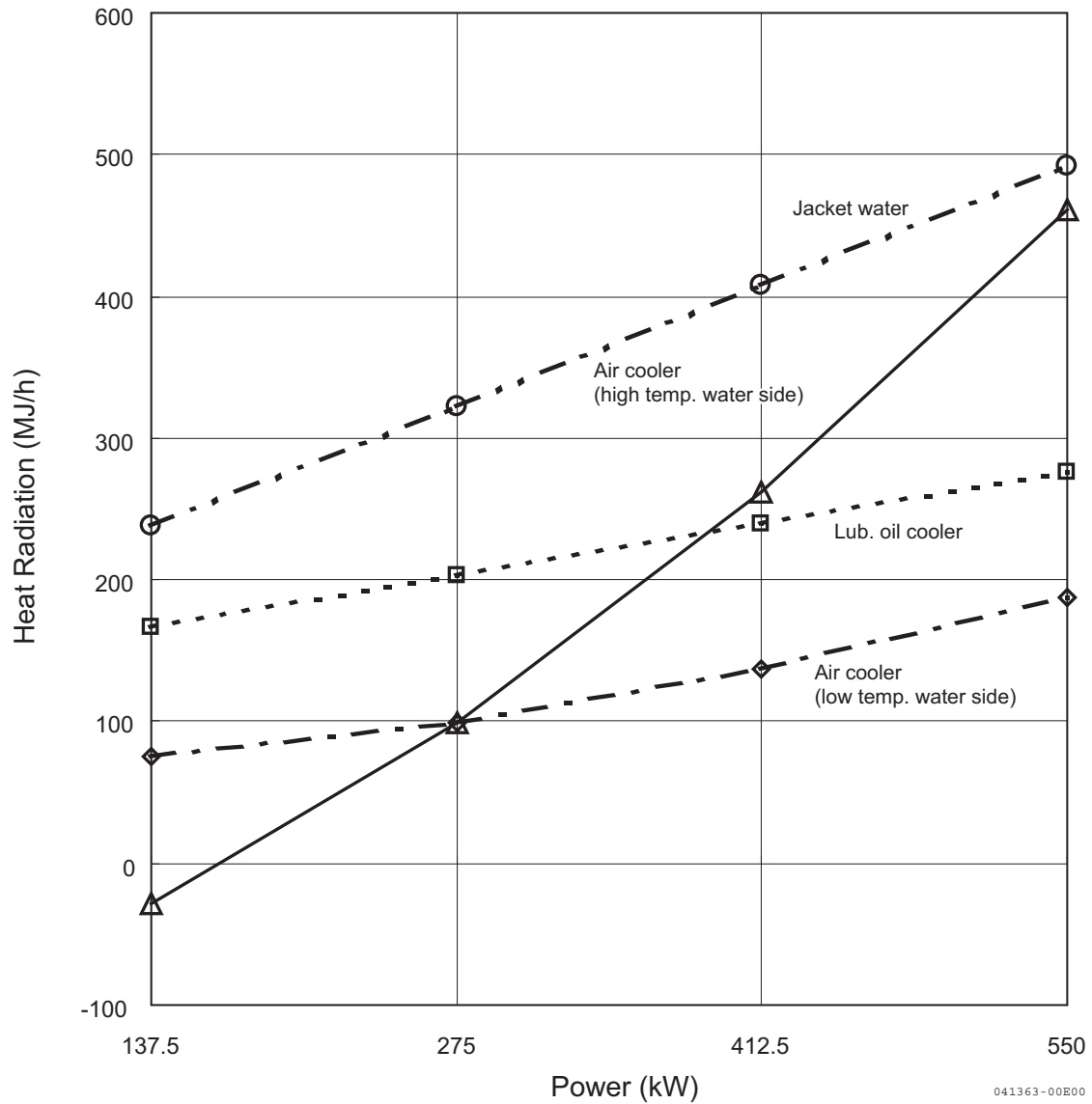
Heat Radiation
